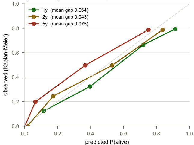
does a stated probability mean what it says? quartiles of predicted survival, hold-out
