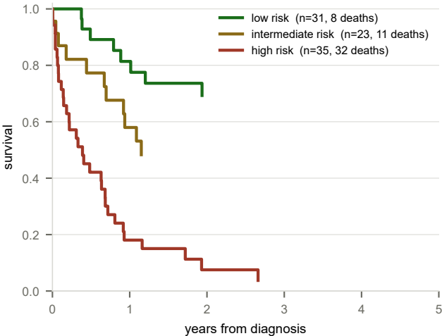
sealed hold-out, split by predicted risk tertile low vs high log-rank p = 2.8\text{e-}09
