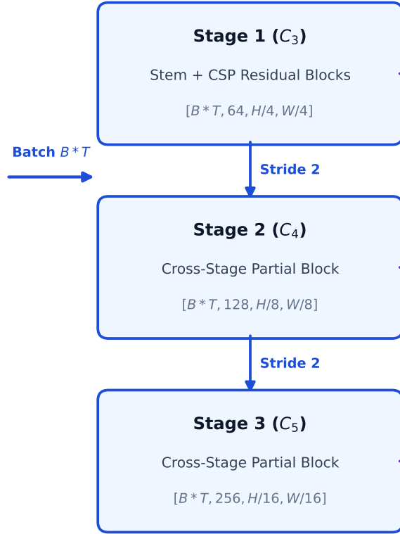
(b) CSP-Darknet Backbone
