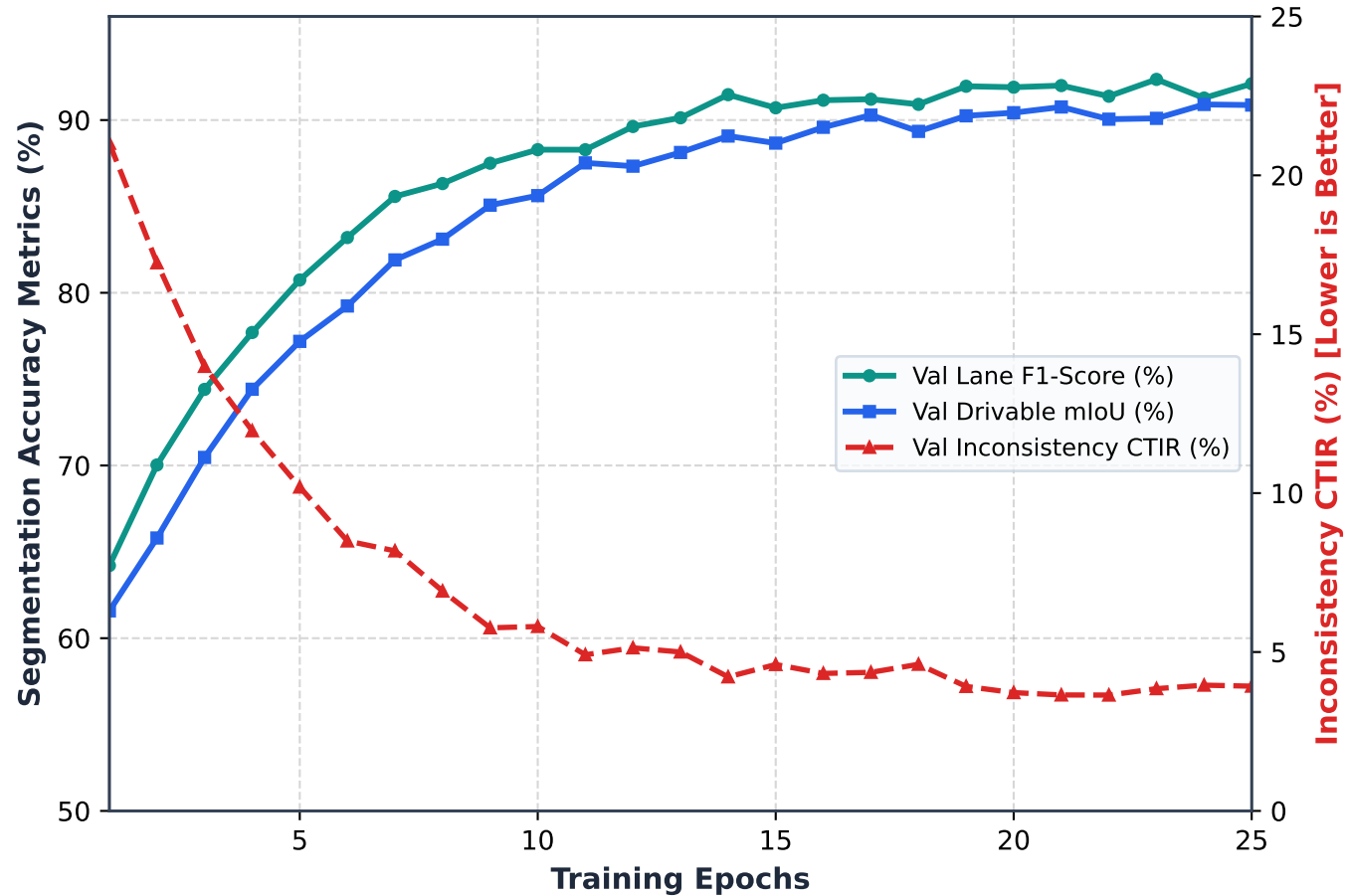
(b) Validation Metrics Evolution over Epochs
