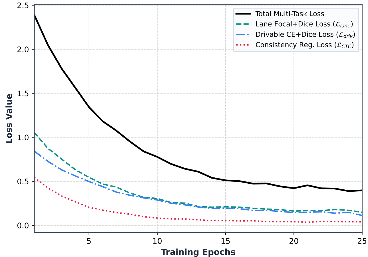
(a) Multi-Objective Loss Convergence Dynamics
