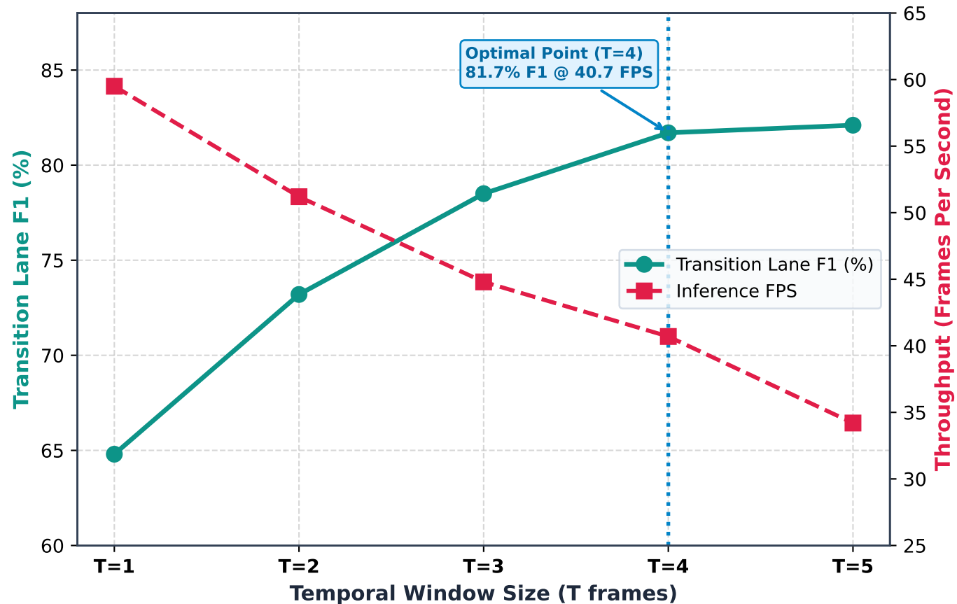
(b) Accuracy vs. Throughput Pareto Curve
