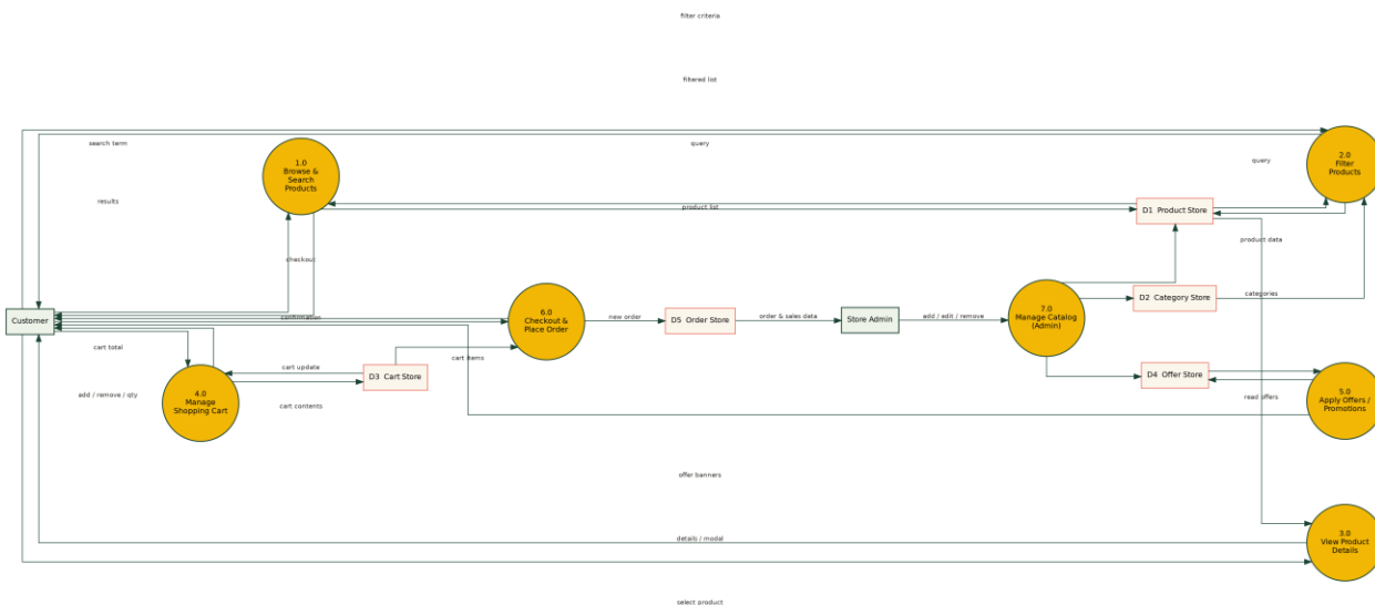
Figure 3 — DFD Level 1
