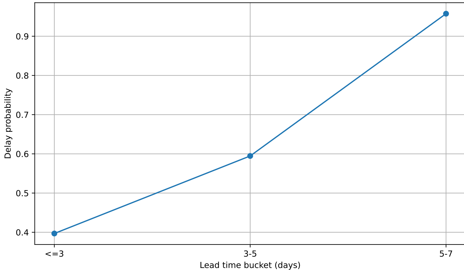
RQ3 - Delay probability by lead time bucket
