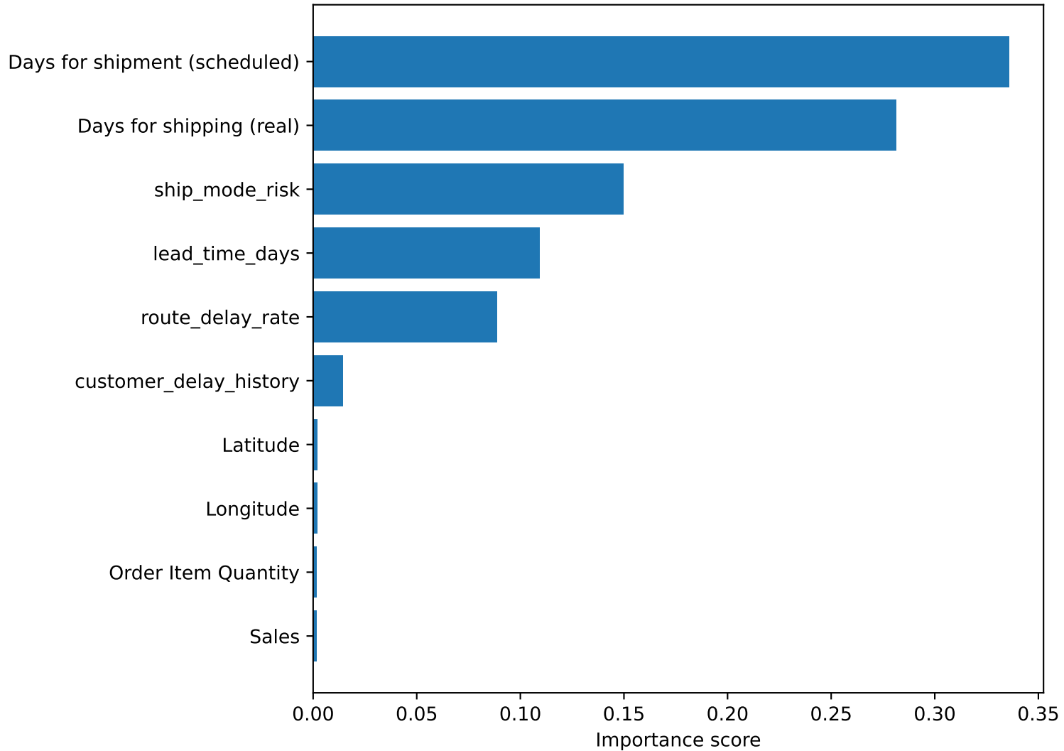
RQ3 - Relative importance of predictors (XGBoost)
