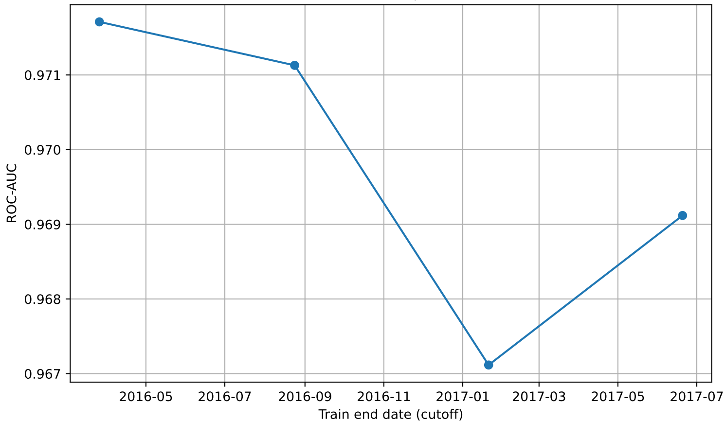
RQ1 - Time-based validation performance (XGBoost)
