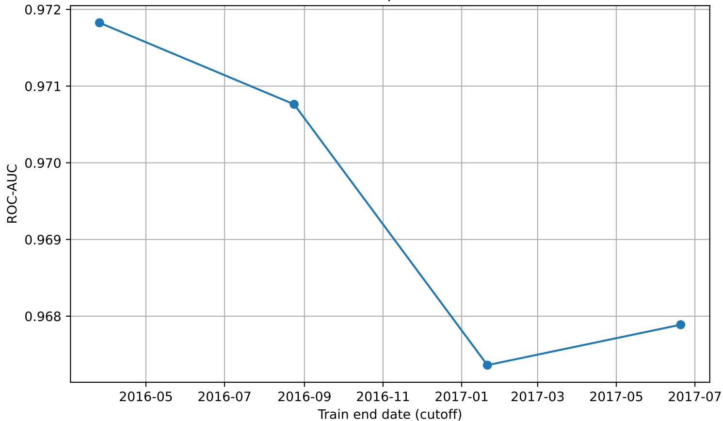
RQ1 - Time-based validation performance (Random Forest)
