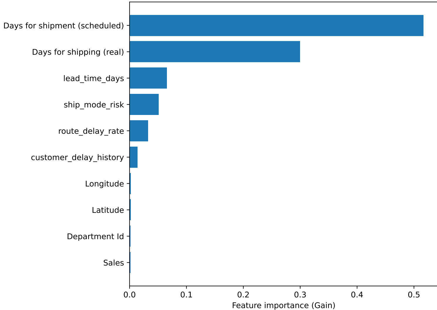
RQ1 - Feature importance (XGBoost)
