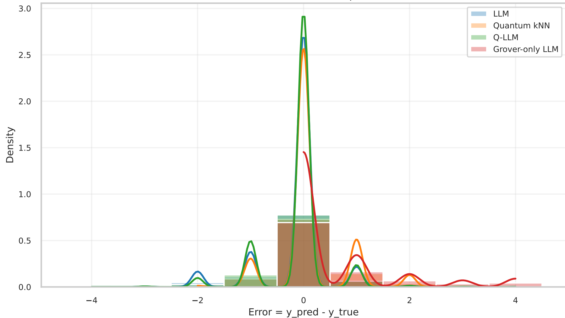
Q-LLM — Error Distribution per Model
