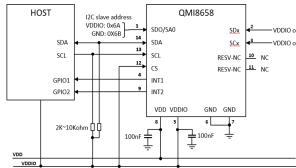
Figure 6. I3C/I 2 C-UI mode
