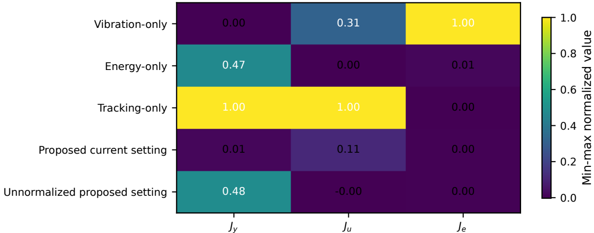
Objective Conflict Under Single-Objective Optima
