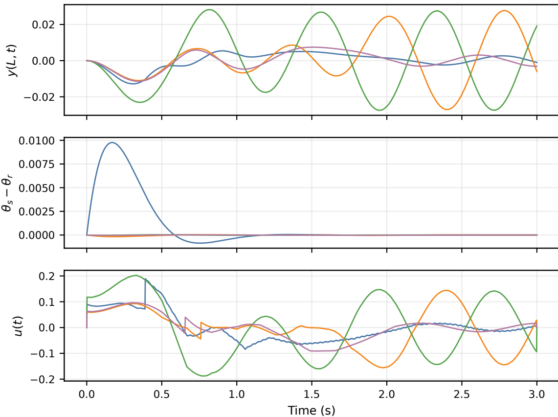
W1 W2 W3 W14 Representative Closed-Loop Responses
