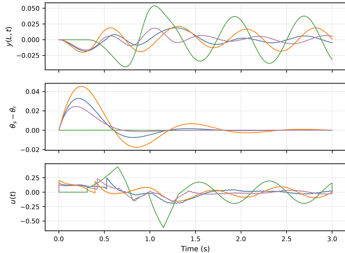
— W1 — W2 — W3 — W14 Representative Closed-Loop Responses
