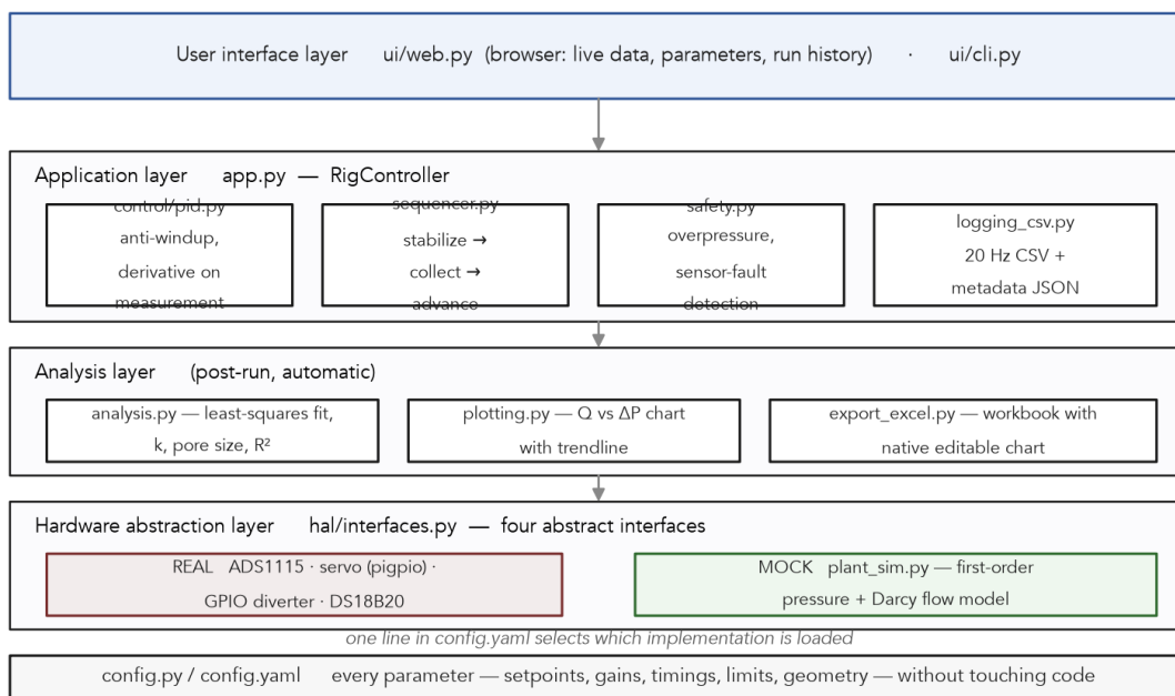
Figure 2. Software layer map. Each box is one module; arrows indicate dependency direction. The hardware abstraction layer is the only code that touches physical devices, so replacing the real drivers with the mock plant exercises everything above it unchanged.
