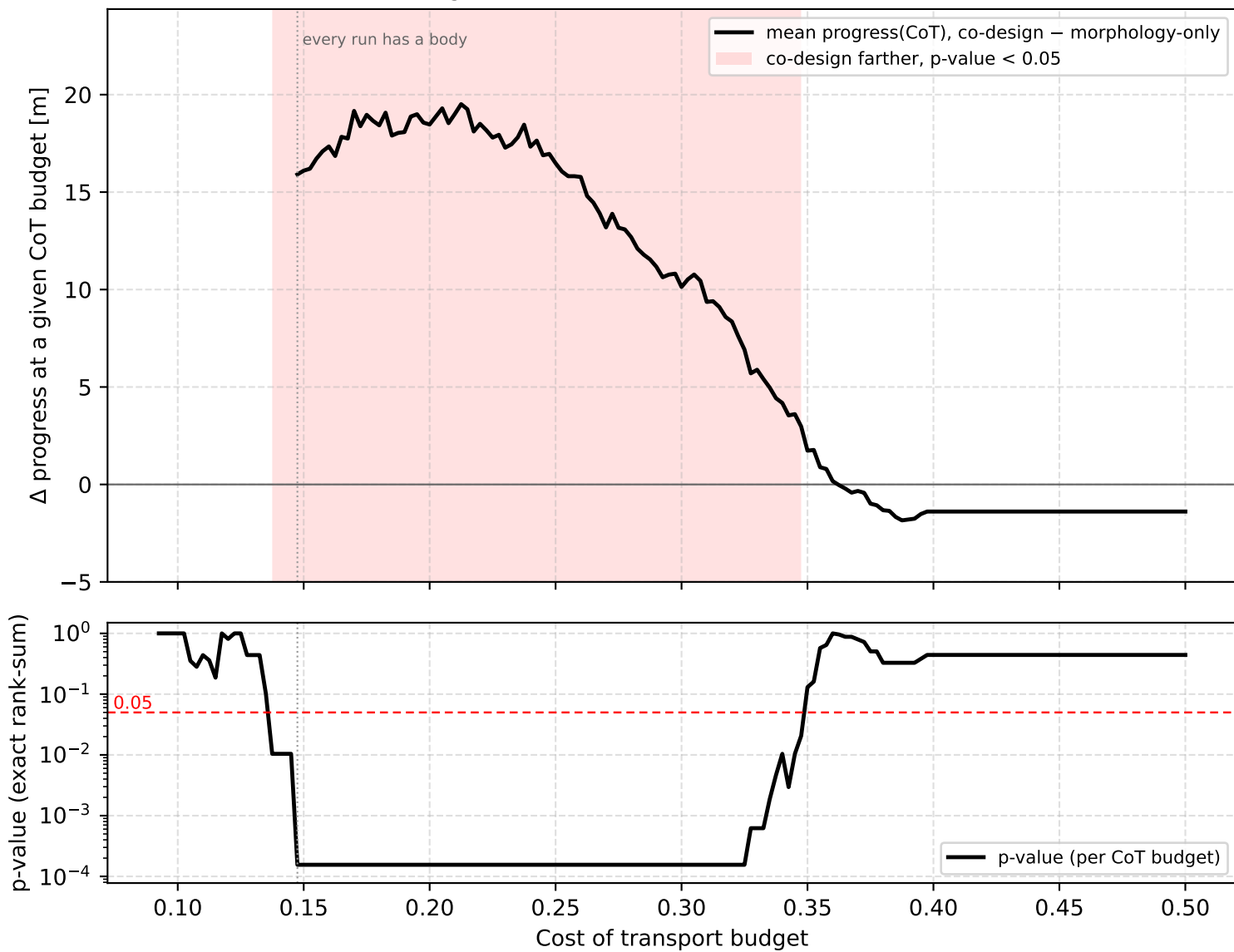
Progress-at-CoT difference between conditions
