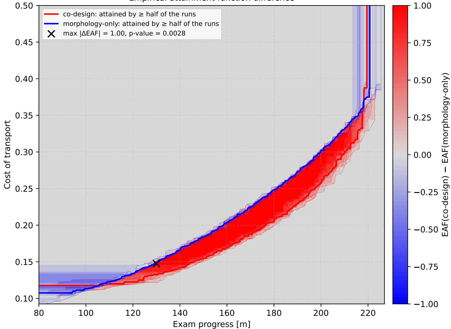
Empirical attainment function difference
