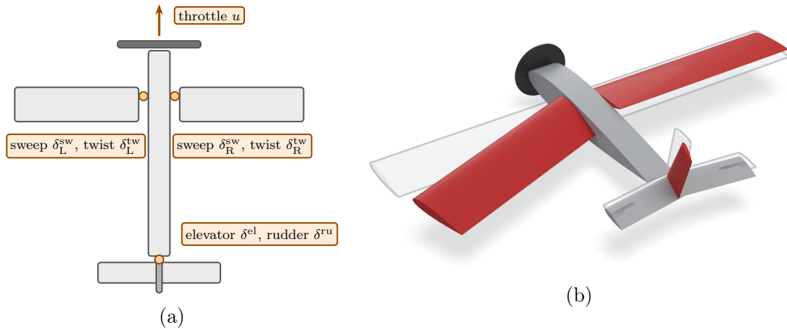
Figure 4.3: Parts and actuators of the drone. (a) The seven commands, on a schematic top view with the nose up: the throttle of the propeller, the sweep and the twist of each wing panel, the elevator and the rudder. (b) The reference drone with the left panel swept back to the limit of its range, the two panels twisted in opposite directions, and the elevator and the rudder deflected; the neutral position of every surface is shown in light grey.
