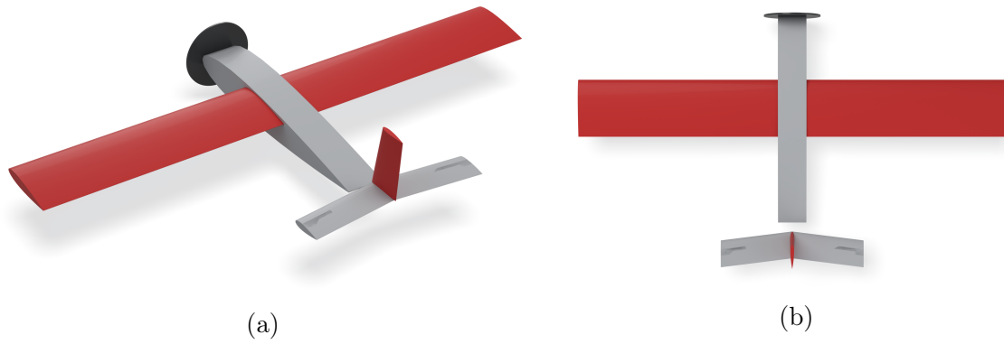
Figure 4.5: The standard drone with all joints in their neutral position: (a) three-quarter view, (b) top view with the nose up. The wing panels and the rudder are drawn in red, the fuselage and the elevator in grey, the disc of the propeller in black.
