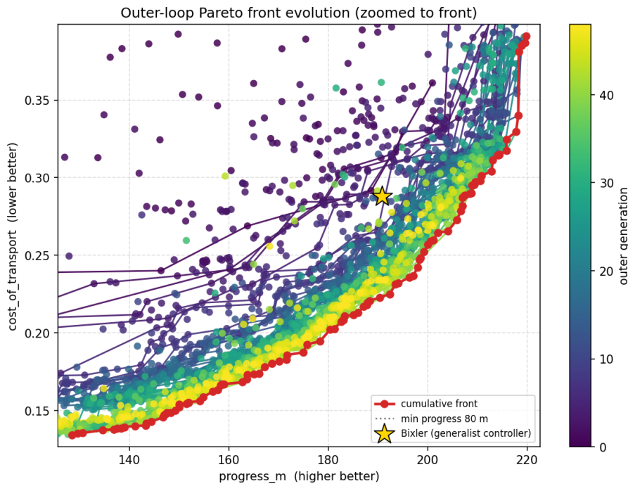
Figure 6.9: The examined bodies of the first co-design run in the plane of the objectives, coloured by the phase of their exam, with the cumulative front of the run in red; bodies below 128 m of progress are left out of the view. The lines join the successive exams of the bodies that survived more than one phase.
