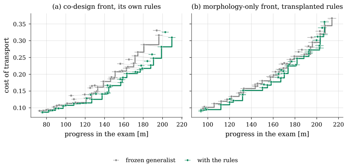
Figure 6.7: The bodies of a last front flown again on the exam course, over the same 256 forests, by the frozen generalist (grey) and by the Hebbian controller with the best set of rules of a co-design run (green); each body is one point in both colours, joined by a dotted line, with the standard error of its progress as a bar, and the steps are the fronts of the two sets of points. (a) A co-design front under its own rules. (b) A morphology-only front under the same rules, transplanted.
