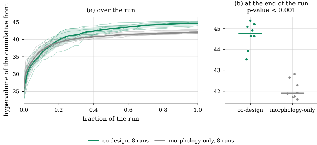
Figure 6.6: Hypervolume of the cumulative fronts, reference point at 80 m and a cost of transport of 0.5. (a) Over the course of the runs, on the axis of the fraction of the run that is completed, since a co-design run holds 50 or 33 exams and a control run 87: thin lines are the single runs, thick lines the mean of each condition with a band of one standard deviation. (b) At the end of the runs, one point per run.
