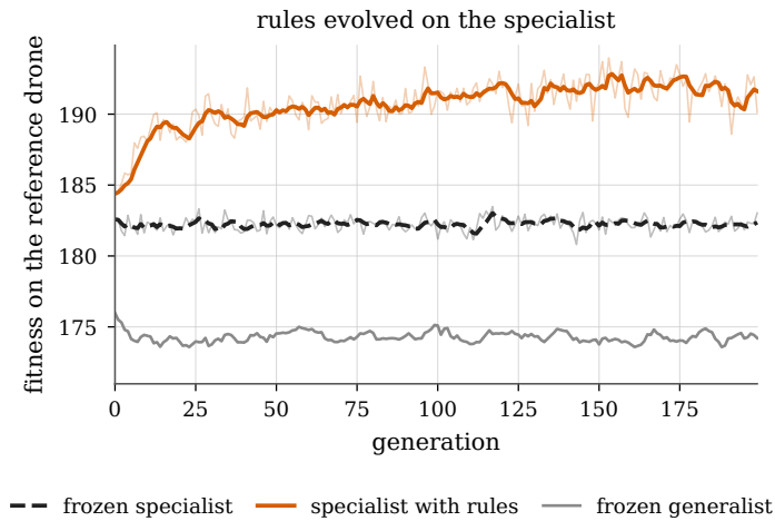
Figure 6.3: The inner loop on the reference drone alone, with the first specialist as base: fitness of the best set of rules of each generation, of that specialist frozen and of the frozen generalist, over 2048 new forests per generation flown by all three. Thin lines are the raw values, thick lines a moving average over five generations.
