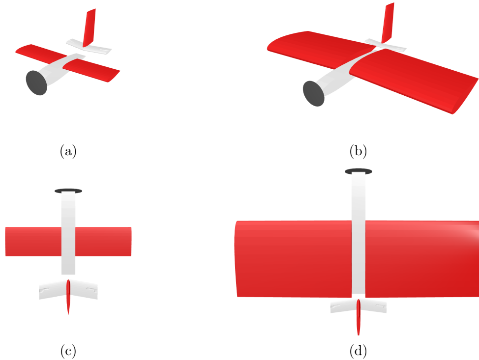
Figure 6.10: The two ends of the front of the first co-design run, drawn at one common scale. Left, (a) and (c): the body that flies farthest. Right, (b) and (d): the cheapest body that passes the gate. Three-quarter views above, top views with the nose up below; wing panels and rudder in red, fuselage and elevator in grey.
