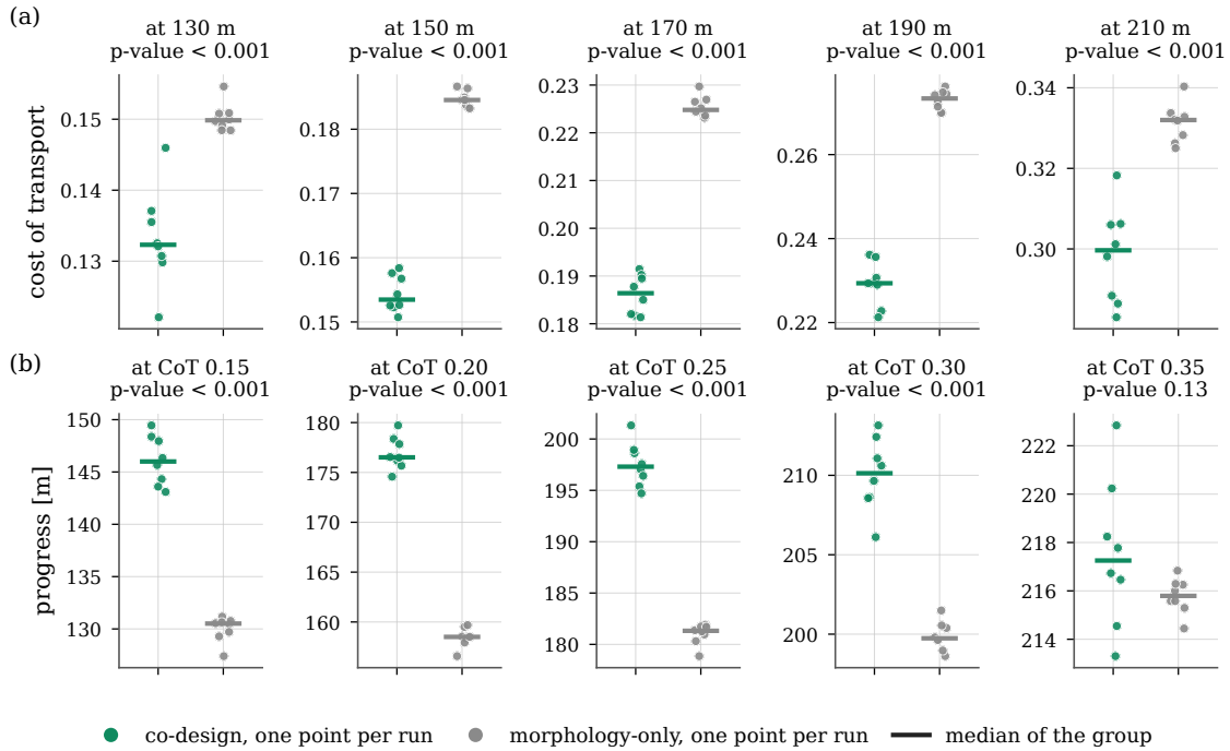
Figure 6.5: The fronts read at fixed progress and at fixed cost of transport, one point per run and the median of each group as a bar. (a) Cost of transport of the cheapest body of the front that reaches 130, 150, 170, 190 and 210 m. (b) Progress of the farthest body of the front within a cost of transport of 0.15, 0.20, 0.25, 0.30 and 0.35. The p-values are those of the exact rank-sum test over the sixteen runs.
