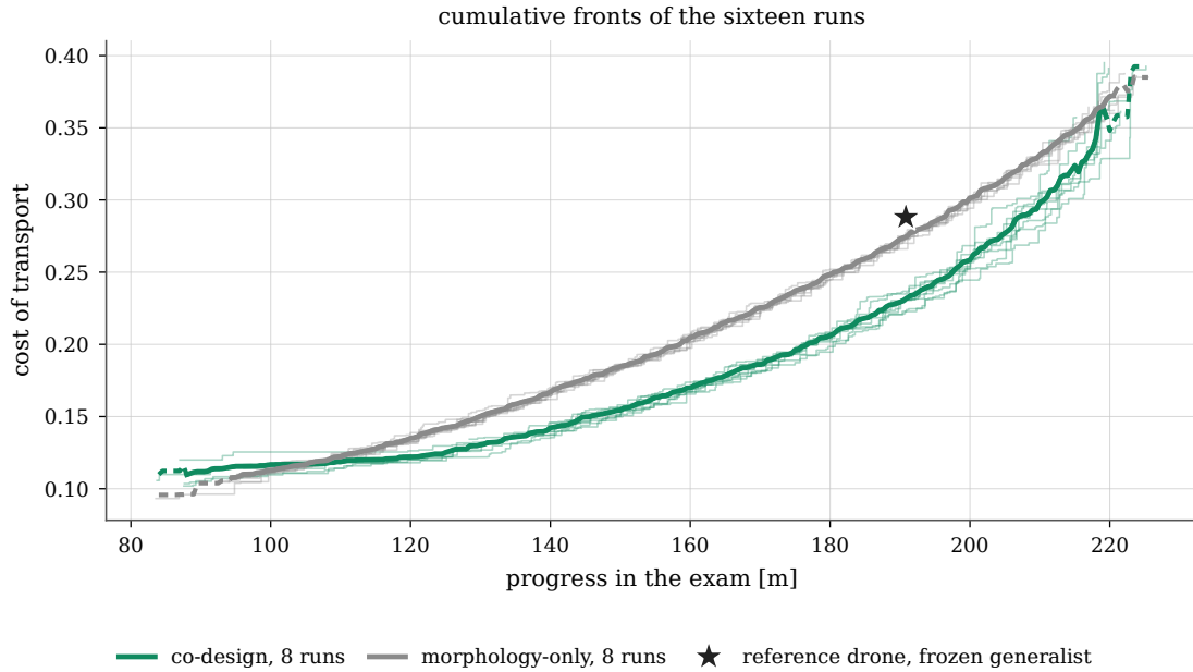
Figure 6.4: The cumulative fronts of the sixteen runs on the exam course, co-design in green and morphology-only in grey. Thin lines are the fronts of the single runs; the thick line of each condition is, at every progress, the mean over its runs of the cost of transport of the cheapest body that reaches that progress, drawn solid where at least four of the eight fronts reach it and dashed where fewer do. The star is the reference drone flown by the frozen generalist.
