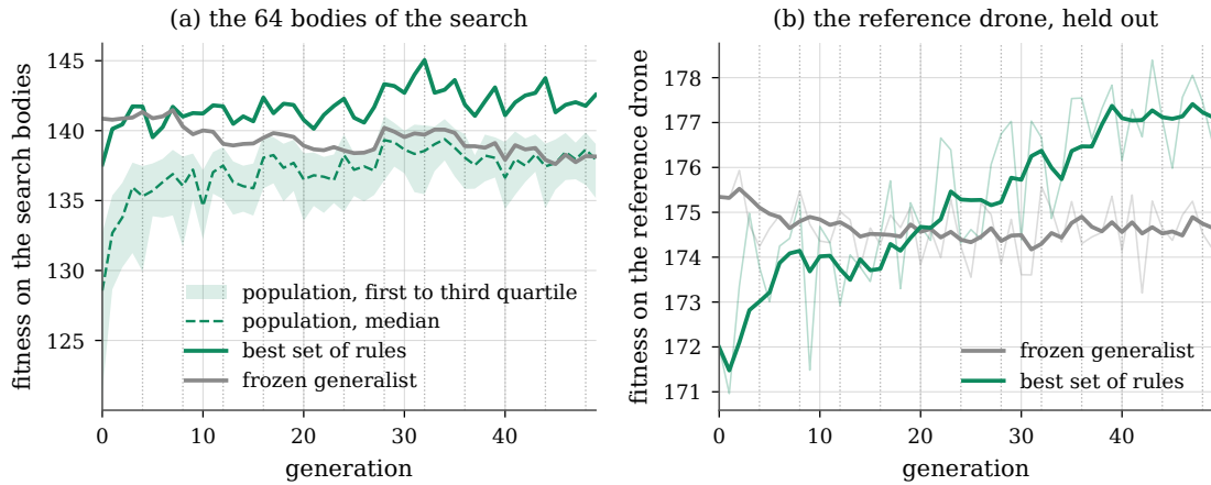
Figure 6.1: The inner loop on 64 random bodies. (a) Fitness on the bodies of the search: the best of the 64 sets of rules of each generation, the population’s median with a band from the first to the third quartile, and the frozen generalist on the same bodies and forests. The dotted lines mark the refreshes of the bodies. (b) The best set of rules of each generation and the frozen generalist on the reference drone, which the search never flies, over 4 096 new forests per generation; thin lines are the raw values, thick lines a moving average over five generations.
