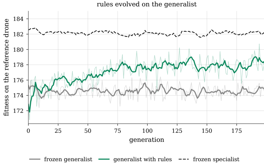
Figure 6.2: The inner loop on the reference drone alone, with the generalist as base: fitness of the best set of rules of each generation, of the frozen generalist and of the frozen specialist, over 2048 new forests per generation flown by all three. Thin lines are the raw values, thick lines a moving average over five generations.
