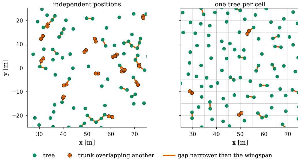
Figure 4.4: Independent and stratified positions at the same density, one tree every 25 \text{ m}^2 , in a window of 50 \text{ m} by 50 \text{ m} with trunks to scale. With independent positions 25% of the trunks overlap another and 64% leave a gap narrower than the width b = 1.4 \text{ m} of the reference drone; with one tree per cell the two figures fall to 6% and 39% (averages over 200 forests).
