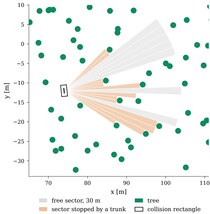
Figure 4.7: What the forest is to the drone, seen from above. The depth sensor divides a fan of 80^\circ ahead of the drone into 20 sectors and reports for each the distance to the nearest trunk, up to 30 m. The collision test of section 4.2 asks whether the centre of a trunk lies inside the rectangle drawn around the wing (trunks and wingspan are to scale).
