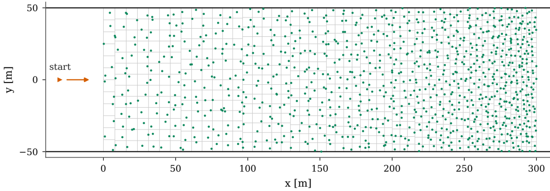
Figure 4.5: A Latin hypercube forest seen from above, with its cells. The cells shrink from 8 m to 3.4 m along the course and each holds exactly one tree, for 988 trees in total, about as many as in Figure 4.2 and Figure 4.3.
