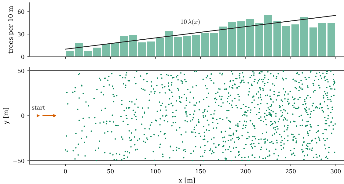
Figure 4.3: A growing density forest seen from above, with \lambda_0 = 1 and \lambda_1 = 5.5 trees per metre over 300 m, which gives the same number of trees, 975, as in Figure 4.2. The upper panel counts the trees in each 10 m of course and compares them with the profile (4.1).
