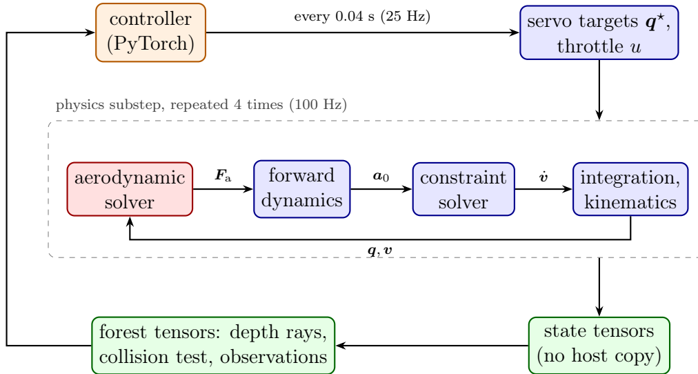
Figure 4.1: One control step. The commands of the controller are held while four physics substeps are executed; in each of them the aerodynamic solver turns the current state into forces, and the rigid body solver of Genesis computes the unconstrained acceleration, enforces the joint limits and integrates. Everything in the figure runs on the GPU, for all environments at once.
