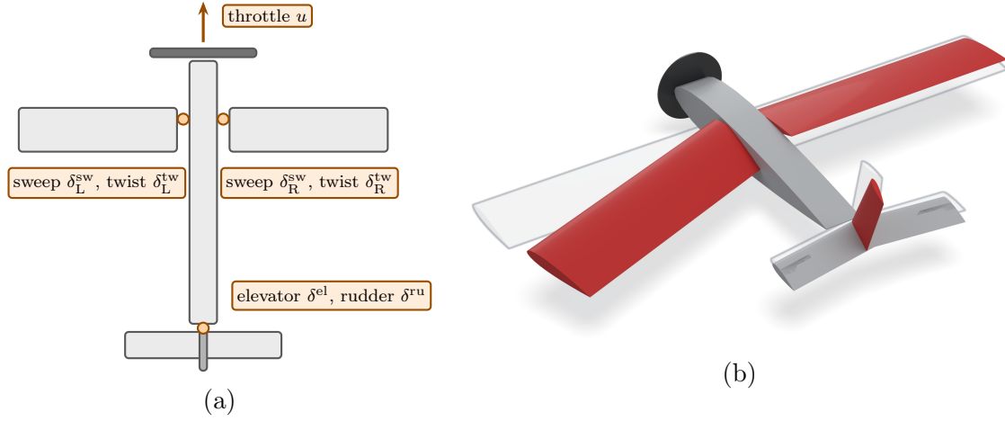
Figure 4.6: Parts and actuators of the drone. (a) The seven commands, on a schematic top view with the nose up: the throttle of the propeller, the sweep and the twist of each wing panel, the elevator and the rudder. (b) The reference drone with the left panel swept back to the limit of its range, the two panels twisted in opposite directions, and the elevator and the rudder deflected; the neutral position of every surface is shown in light grey.
