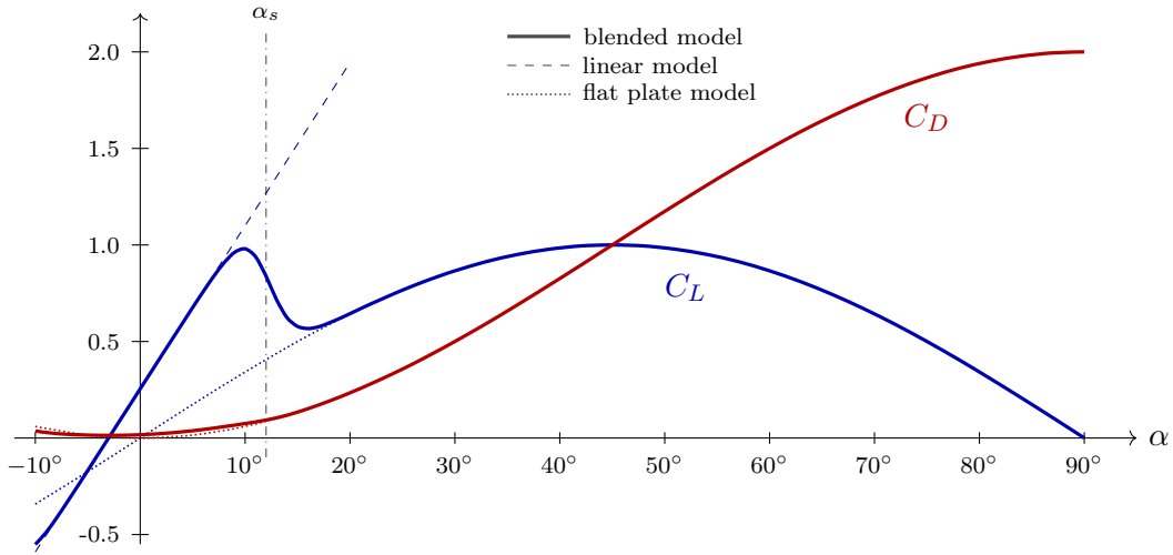
Figure A.2: Lift and drag coefficients of the aerodynamic model for the wing of the reference drone (NACA 3416 section, aspect ratio 7.5). The dashed line is the linear model (A.7) (shown for the lift only), the dotted lines are the flat plate model (A.8), and the solid lines are their blend (A.9) around the stall angle \alpha_s = 12.0^\circ of the finite wing. The maximum lift coefficient is 0.98 and the best lift to drag ratio of the isolated wing is 18.7.
