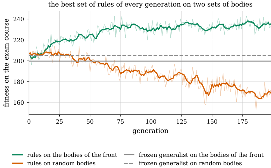
Figure 6.12: The best set of rules of every generation of the first co-design run, flown on the 37 bodies of the run’s last front (green) and on 128 bodies drawn at random from the design space (orange), over the same 64 forests of the exam course for every controller: fitness, mean over the bodies; thin lines are the raw values, thick lines a moving average over five generations. The grey lines are the frozen generalist on the same bodies and forests.
