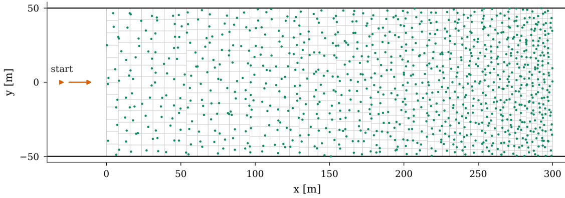
Figure A.5: A Latin hypercube forest seen from above, with its cells. The cells shrink from 8 m to 3.4 m along the course and each holds exactly one tree, for 988 trees in total, about as many as in Figure A.3 and Figure 4.2.
