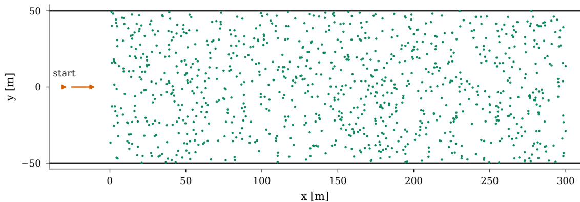
Figure A.3: A uniform density forest seen from above: 975 trees placed independently and uniformly in a corridor of 300 m by 100 m. Trunks are drawn to scale. The thickets and the clearings are what independent positions look like.
