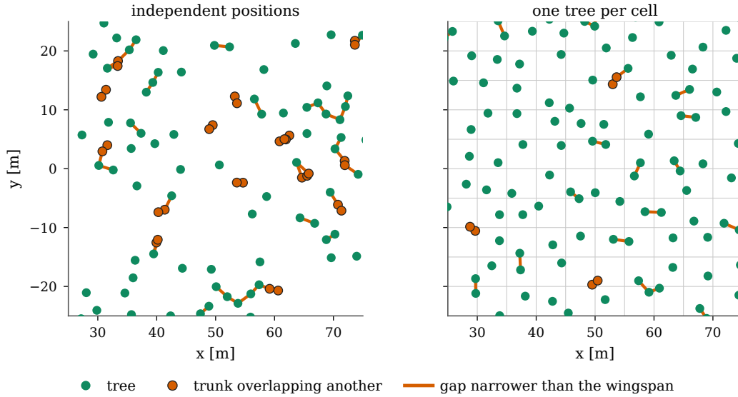
Figure A.4: Independent and stratified positions at the same density, one tree every 25 \text{ m}^2 , in a window of 50 \text{ m} by 50 \text{ m} with trunks to scale. With independent positions 25% of the trunks overlap another and 64% leave a gap narrower than the width b = 1.4 \text{ m} of the reference drone; with one tree per cell the two figures fall to 6% and 39% (averages over 200 forests).
