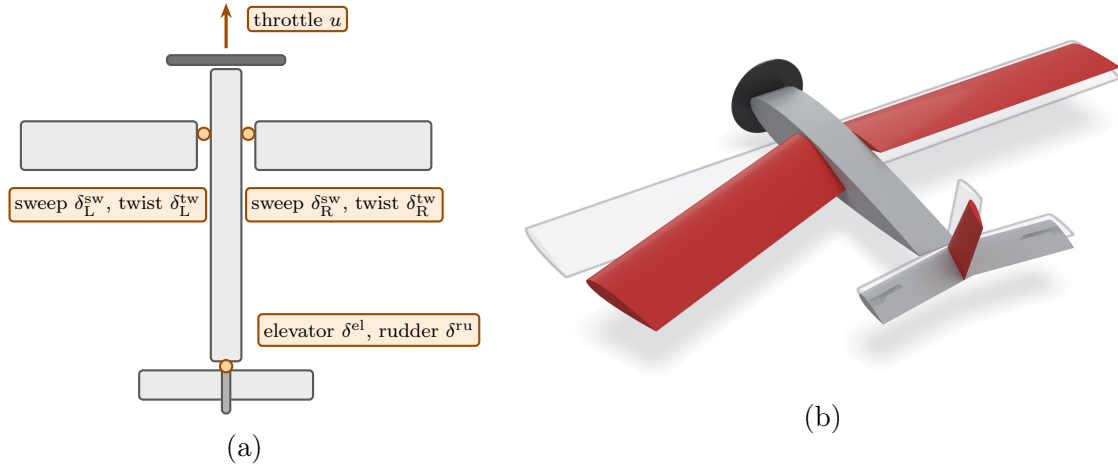
Figure 4.3: Parts and actuators of the drone. (a) The seven commands, on a schematic top view with the nose up: the throttle of the propeller, the sweep and the twist of each wing panel, the elevator and the rudder. (b) The reference drone with the left panel swept back to the limit of its range, the two panels twisted in opposite directions, and the elevator and the rudder deflected; the neutral position of every surface is shown in light grey.
