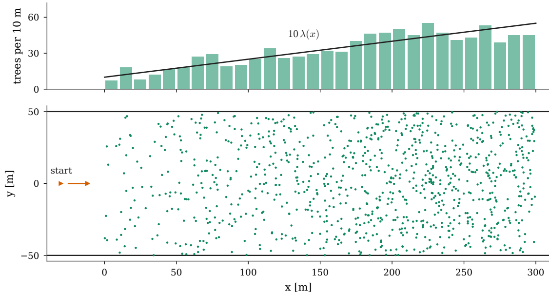
Figure 4.2: A growing density forest seen from above, with \lambda_0 = 1 and \lambda_1 = 5.5 trees per metre over 300 m, for 975 trees in total. The upper panel counts the trees in each 10 m of course and compares them with the profile (4.1).
