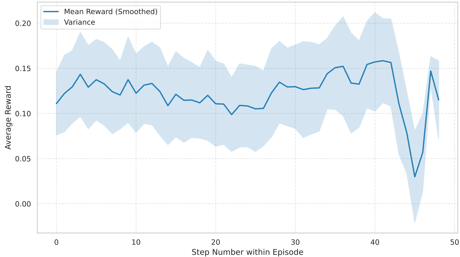
Mean Reward Evolution over Episode Steps
