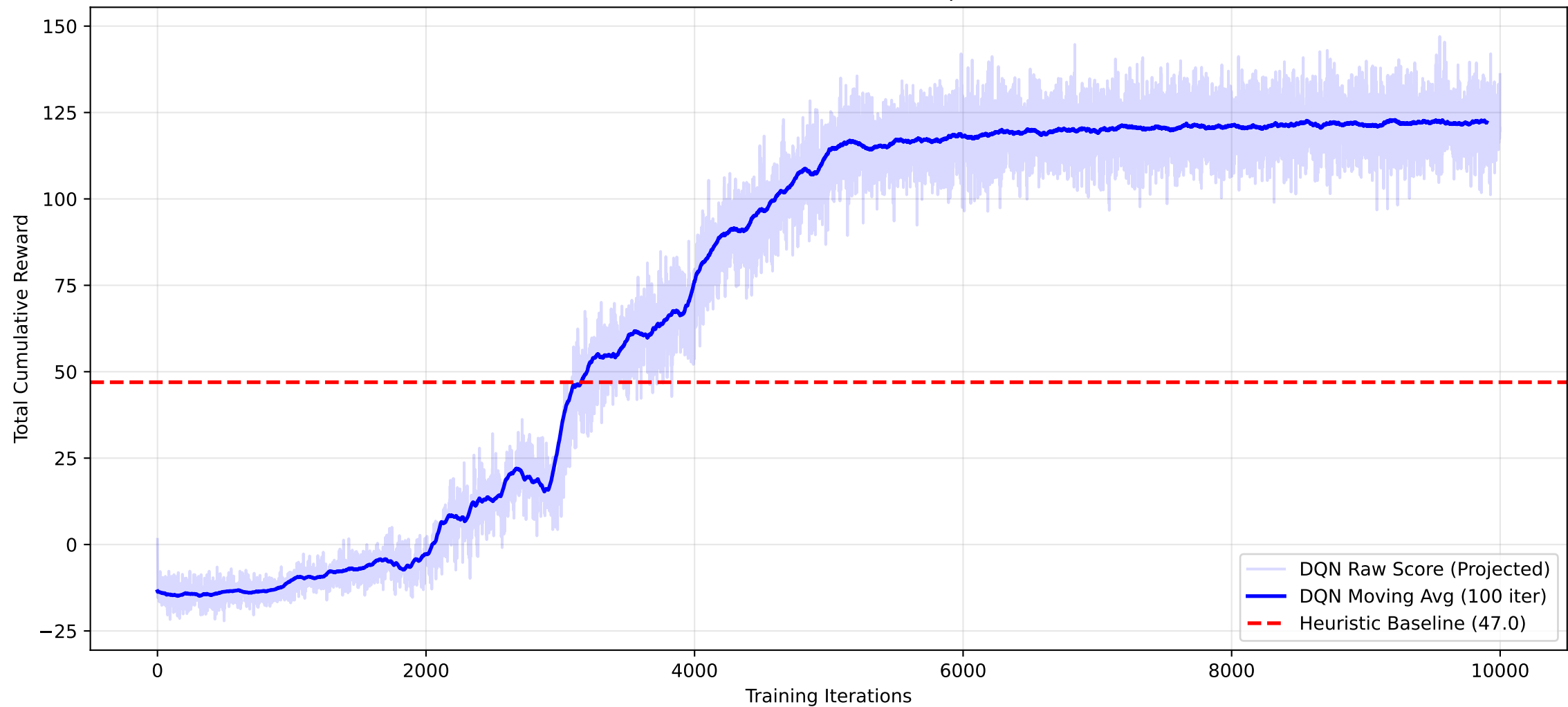
DQN Agent vs Heuristic Baseline (Normalized on 1000 steps)
