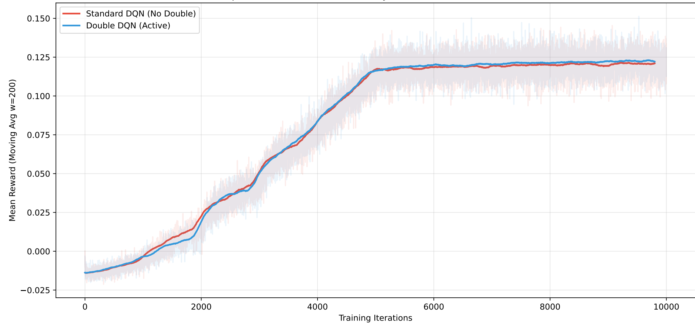
Impact of Double DQN in Fully Observable Environment
