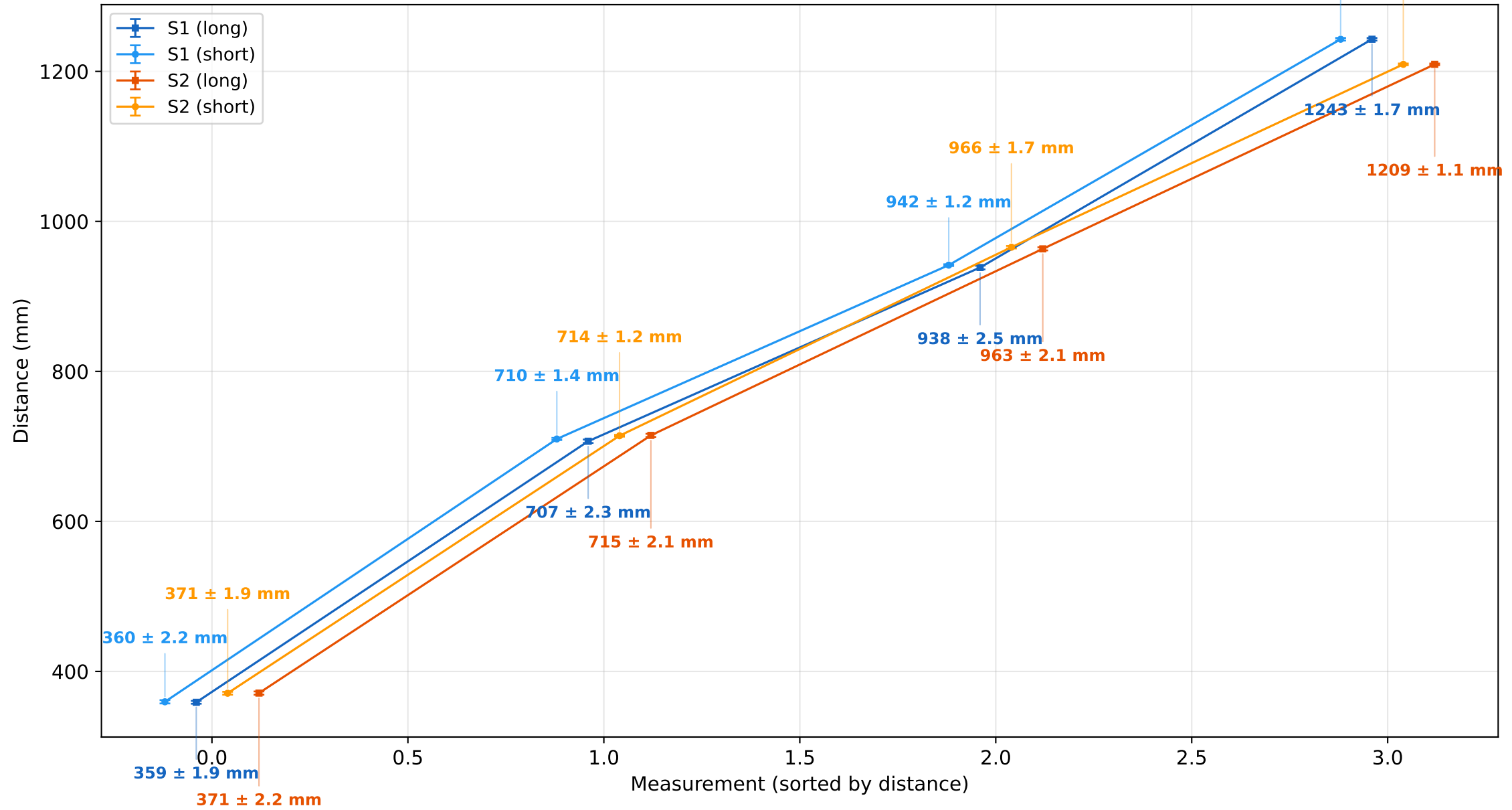
ToF Short vs Long Mode — Both Sensors (mean \pm 1\sigma )
