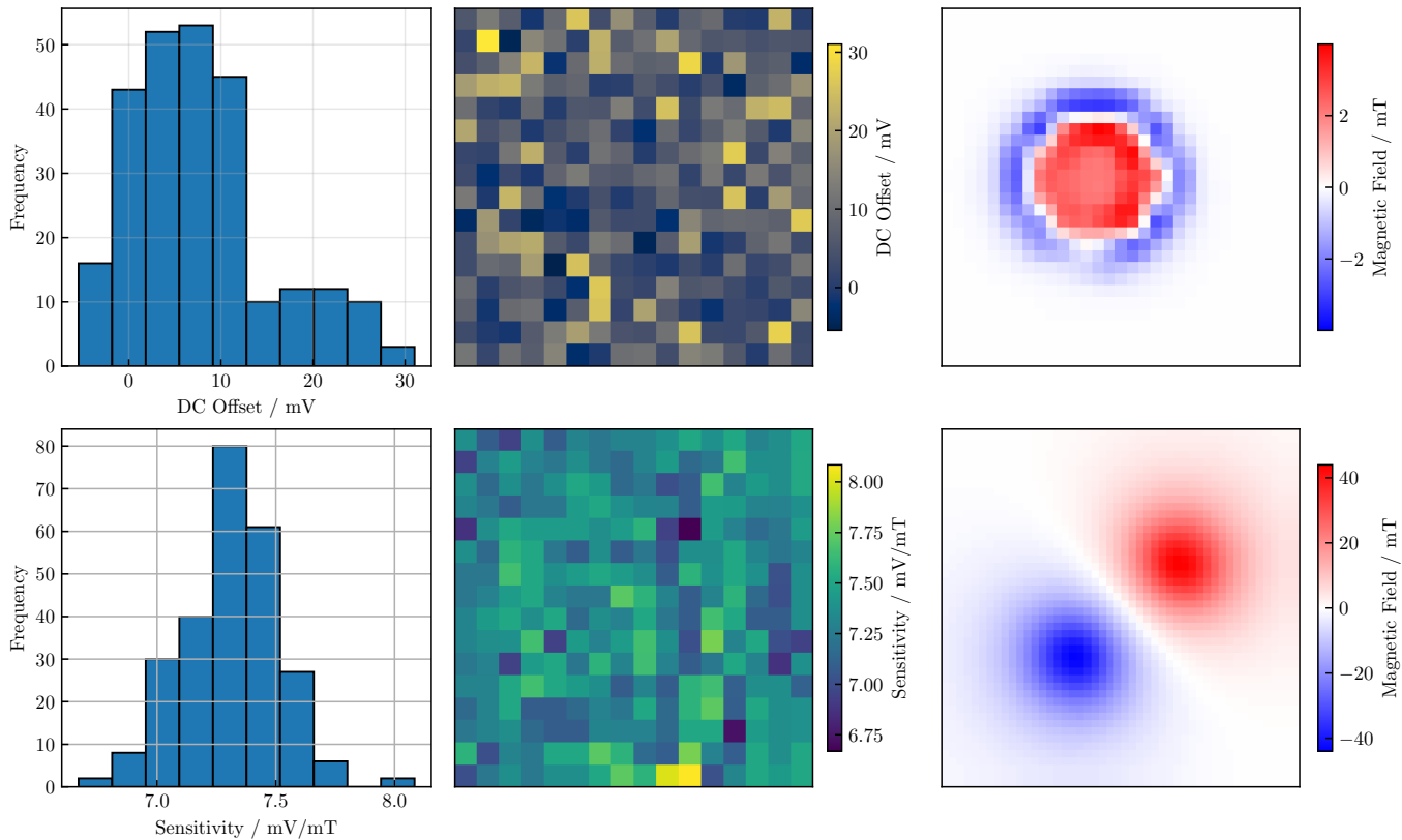
Fig. 14. Calibration results: DC offset with zero applied field (top); linear magnetic field sensitivity (bottom); preliminary imagery (right) of an Apple MagSafe charger and a very strong bar magnet, showing the use of bicubic interpolation. The manufacturer quotes an expected sensitivity of 7.5 mV/mT [19].
