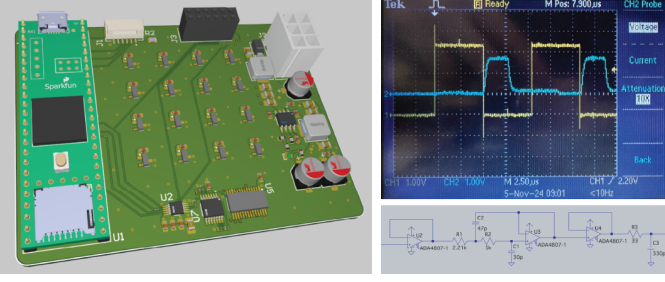
Fig. 11. 1/16th Scale Prototype, with experimental filter testing results and filter schematic shown.
