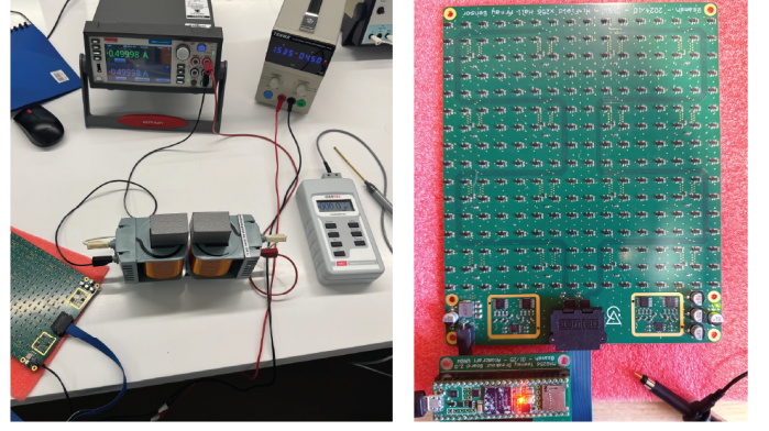
Fig. 12. Linearity calibration setup with source meter, gauss meter, and ferrite core electromagnet (left), and close-up of the completed device (right) with the Teensy digital controller board partially shown.
