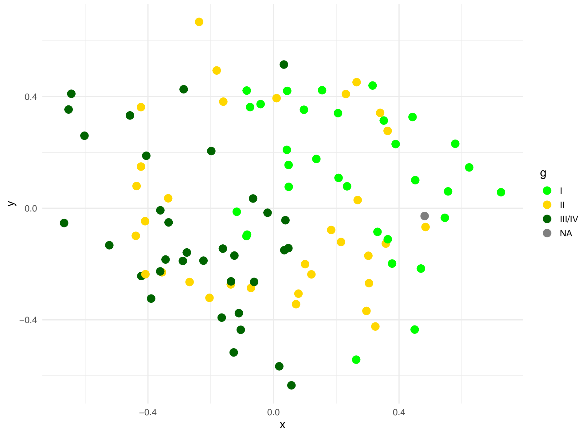
Figure 1D: 4D PCA (Tiers as clusters)
