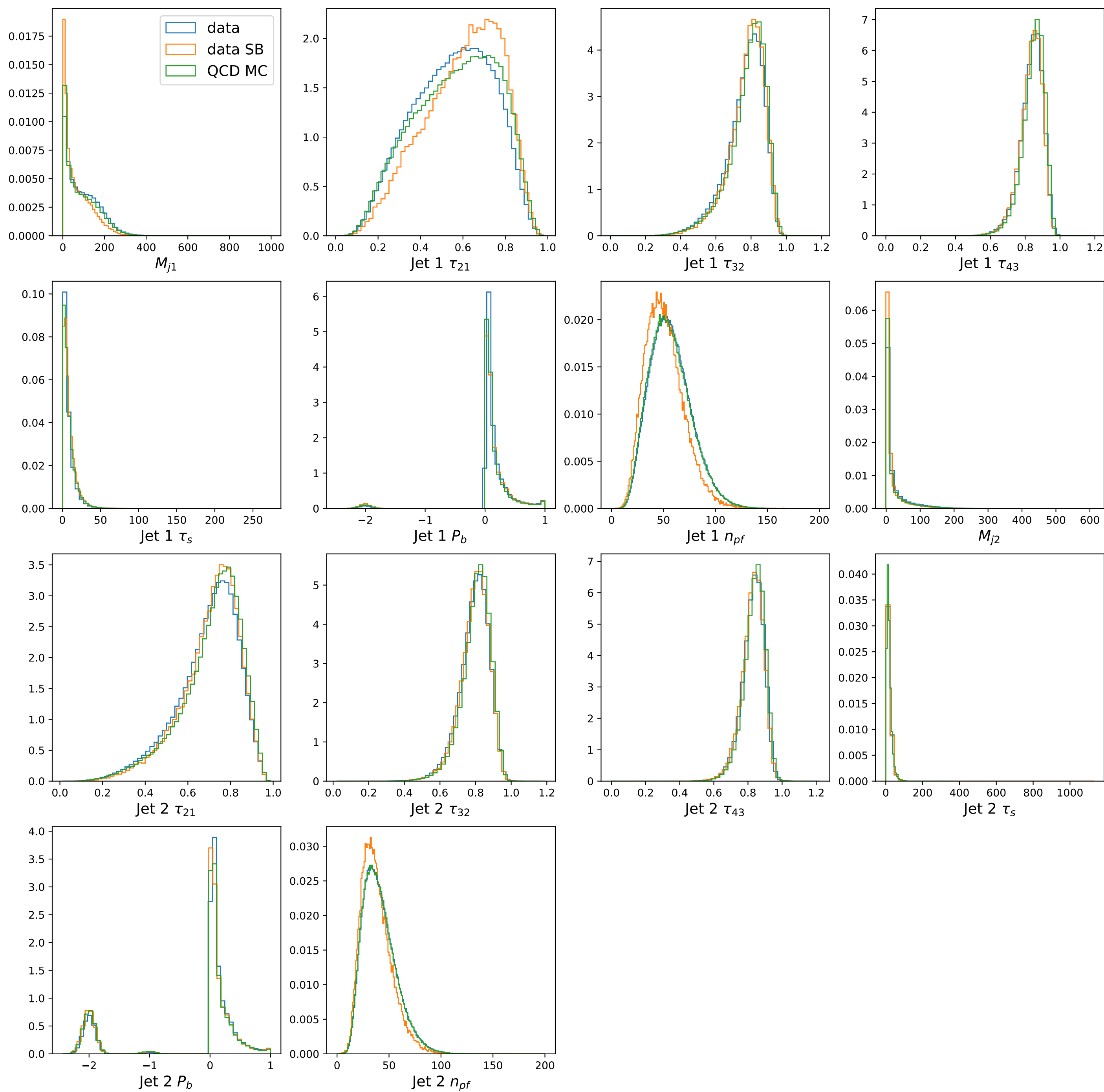
Training Inputs, Data vs QCD MC
