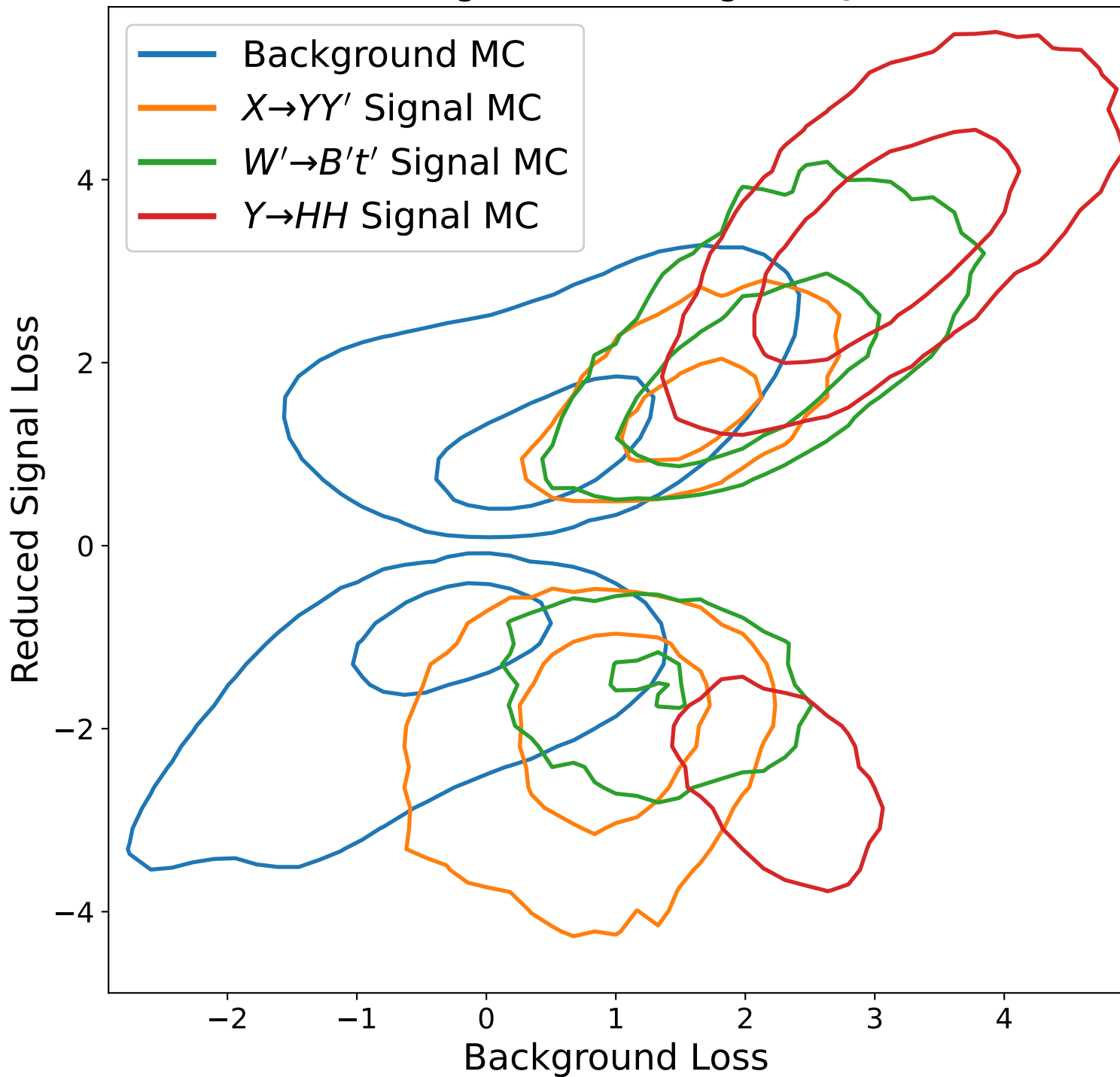
Mass-Binned Signal Axes + Signed L_5 Reduction
