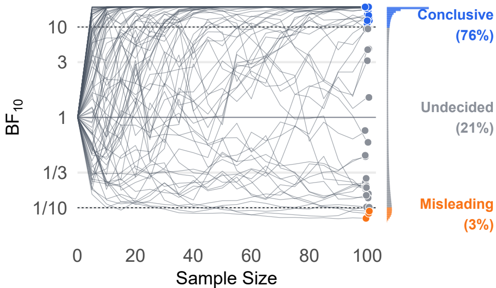
Under H_1
