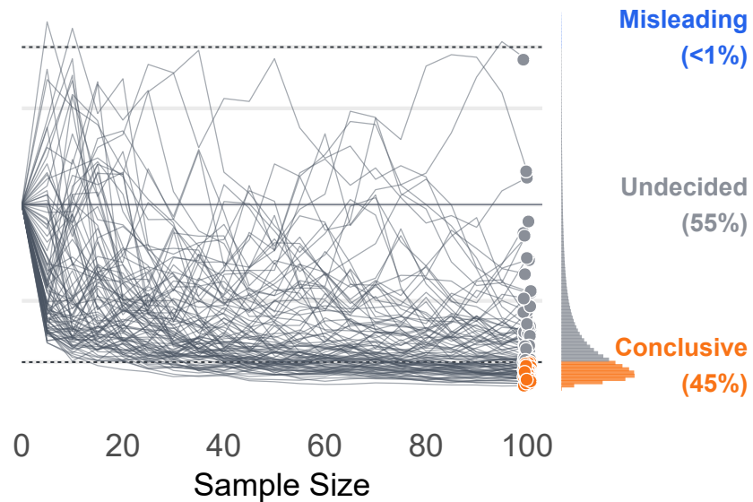
Under H_0
