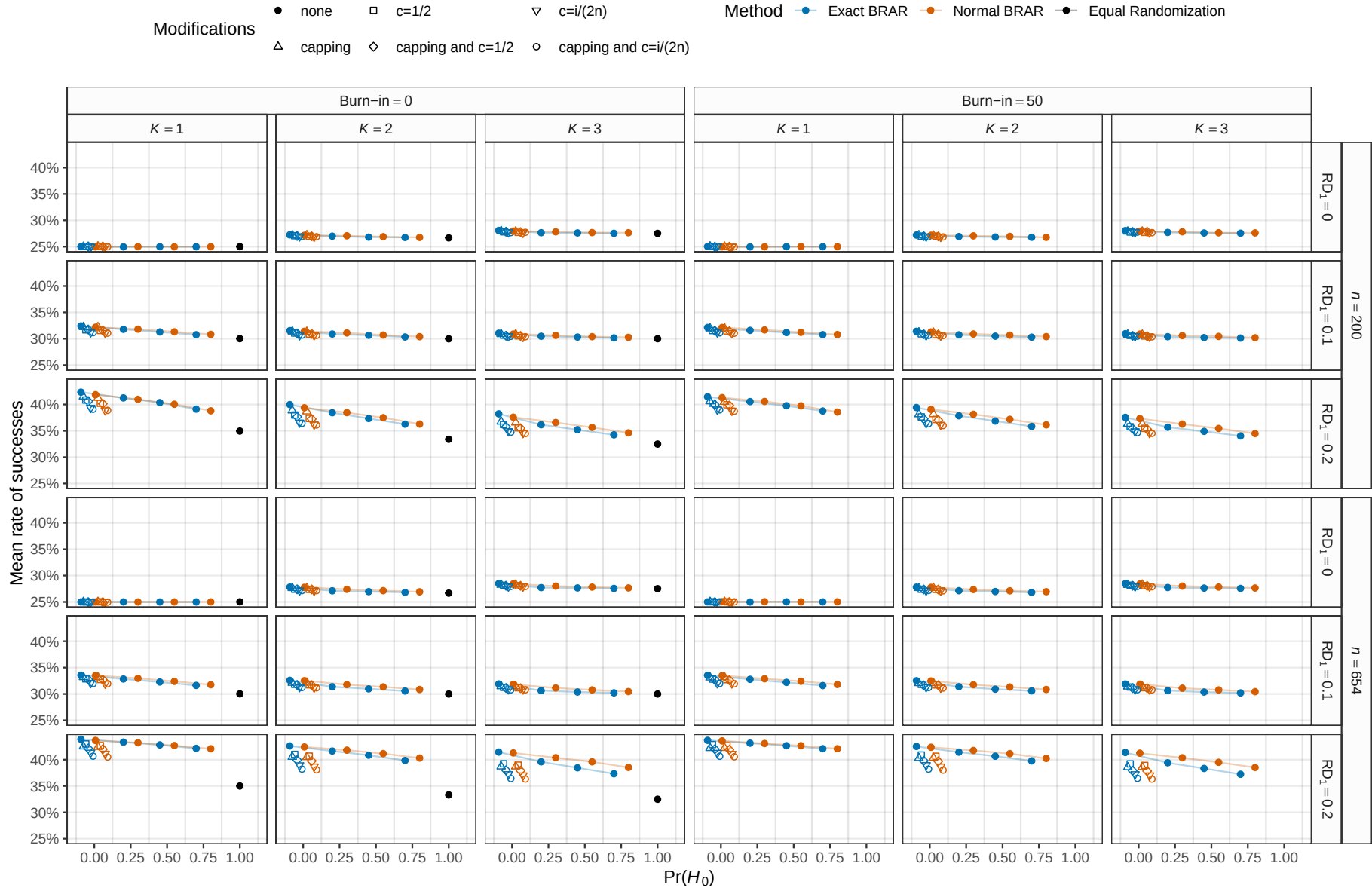
Figure 7: Mean rate of successes (i.e., the number of successes in a study divided by its sample size averaged over all 10'000 simulation repetitions). The maximum MCSE is 0.047%.
