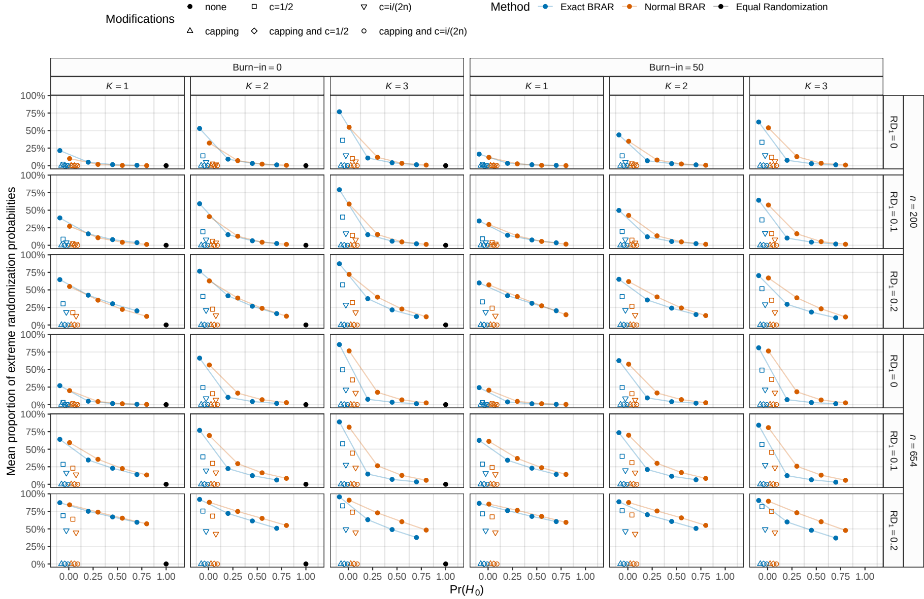
Figure 8: Mean proportion of 10'000 simulations with randomization probabilities either less than 10% or greater than 90%. The maximum MCSE is 0.33%.
