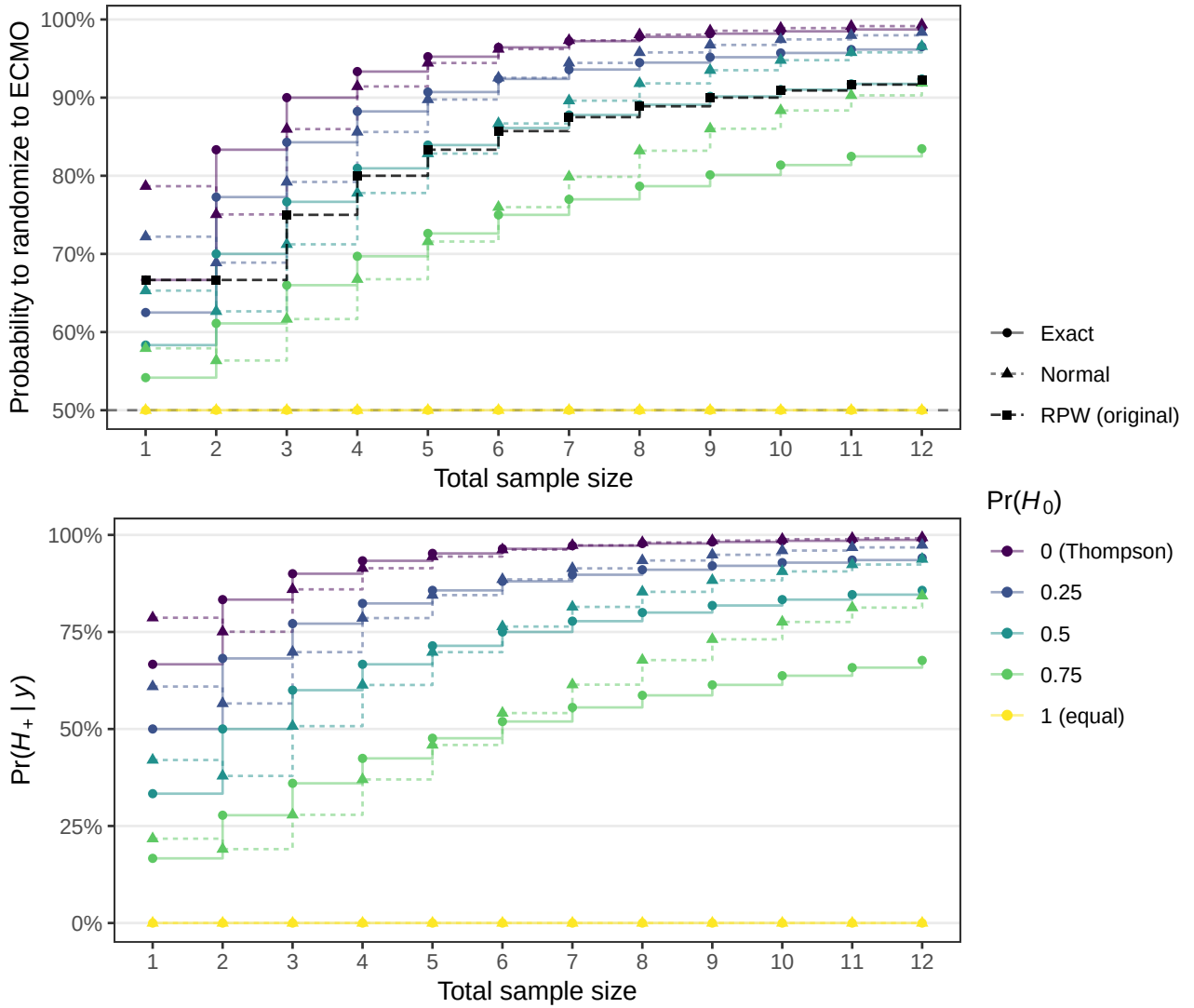
Figure 6: Evolution of Bayesian RAR randomization probabilities (top plot) and posterior probability of a beneficial ECMO treatment effect (bottom plot) for data from the ECMO trial.
