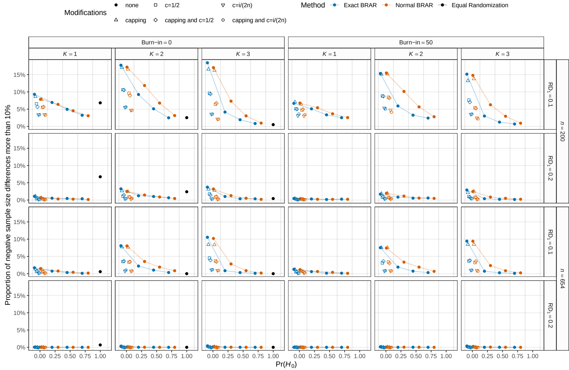
Figure 9: Proportion of 10'000 simulations with more than 10% of the sample size randomized to other groups than treatment group 1. The maximum MCSE is 0.5%.
