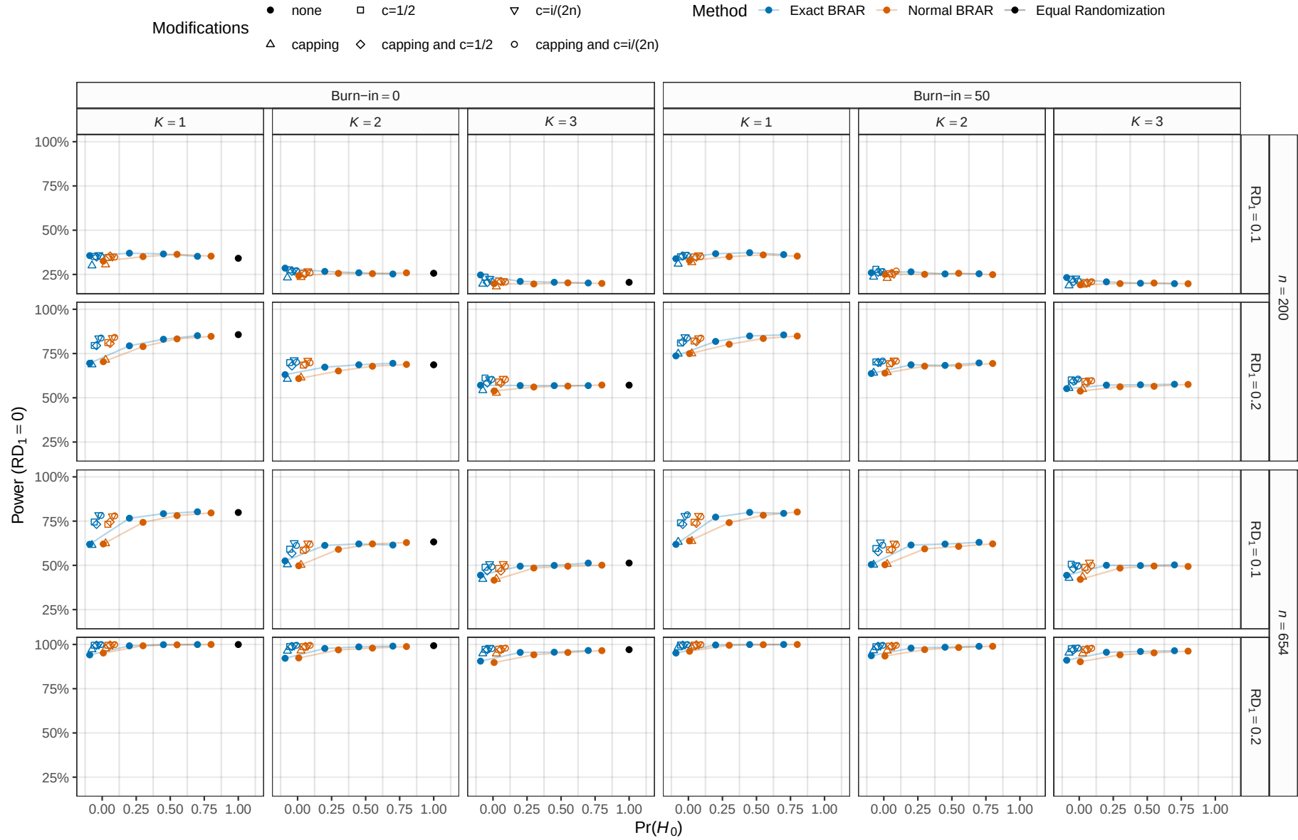
Figure 13: Empirical power of the Wald test of RD_1 = 0 based on 10'000 simulation repetitions. The maximum MCSE is 0.5%.
