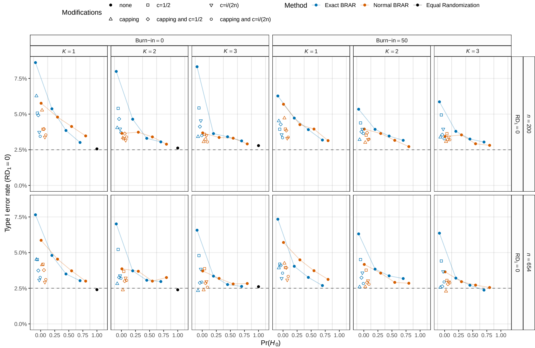
Figure 12: Empirical type I error rate of the Wald test of RD_1 = 0 based on 10'000 simulation repetitions. The maximum MCSE is 0.28%.
