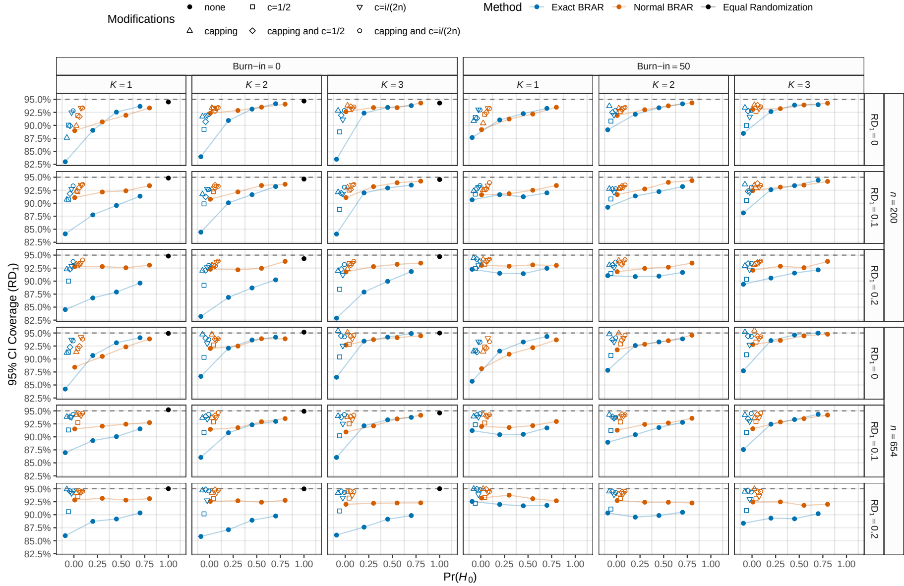
Figure 11: Empirical coverage of the 95% Wald confidence interval for the risk difference RD_1 based on 10'000 simulation repetitions. The maximum MCSE is 0.38%.
