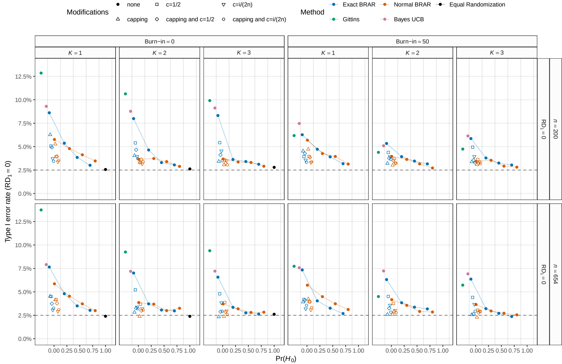
Figure 15: Empirical type I error rate of the Wald test of RD_1 = 0 based on 10'000 simulation repetitions. The maximum MCSE is 0.34%.
