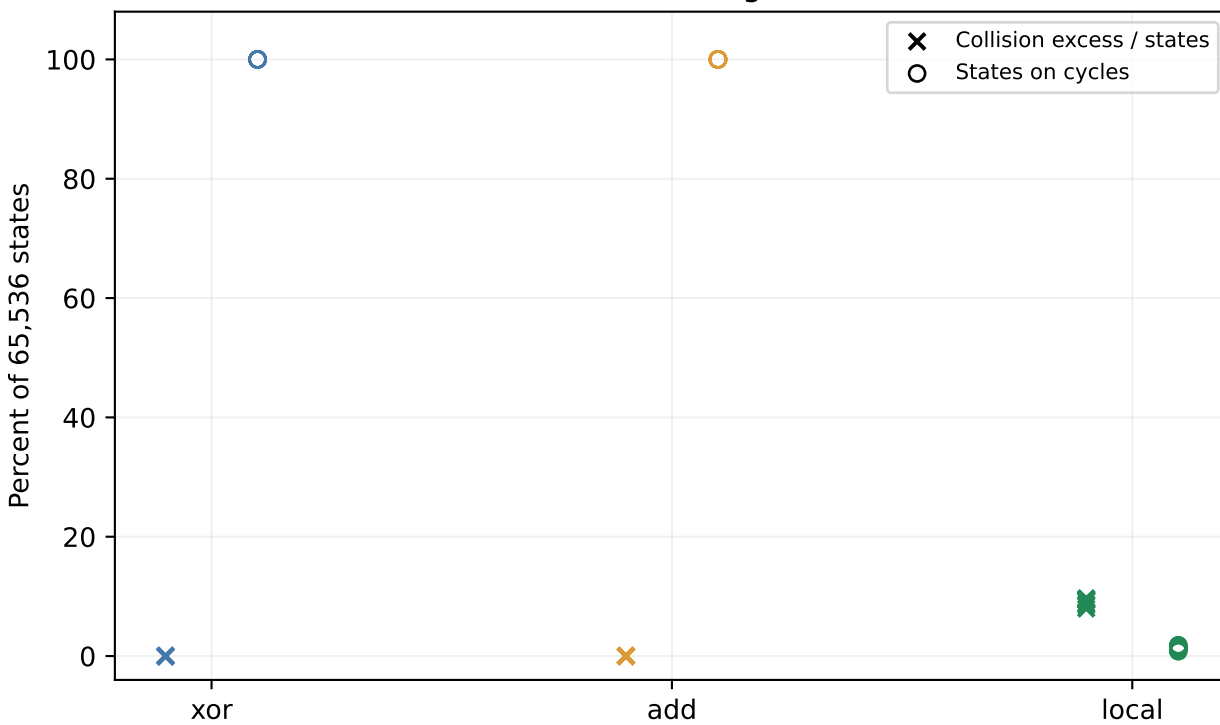
Exhaustive 16-bit analogues: all seeds
