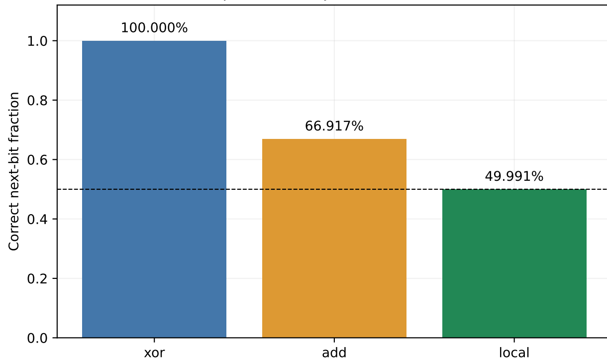
Old predictor: adjacent atoms, 1 MB
