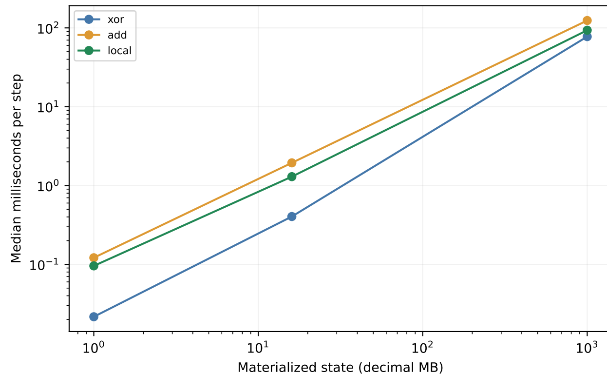
Matched full-state cost: one CPU thread
