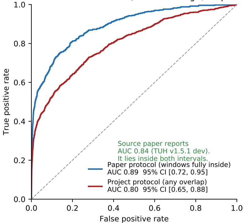
Window-level discrimination, 206 recordings / 28 patients
