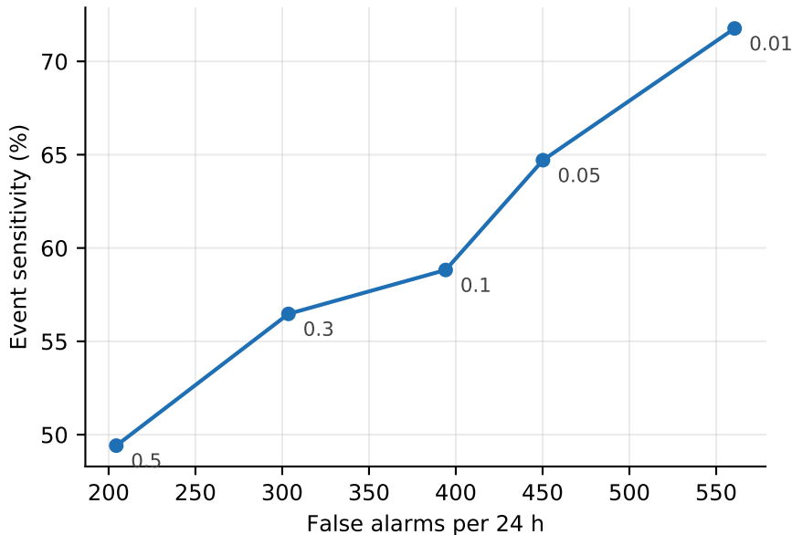
Operating points (labels are detection thresholds) 206 recordings, 27.8 h, 85 seizures
