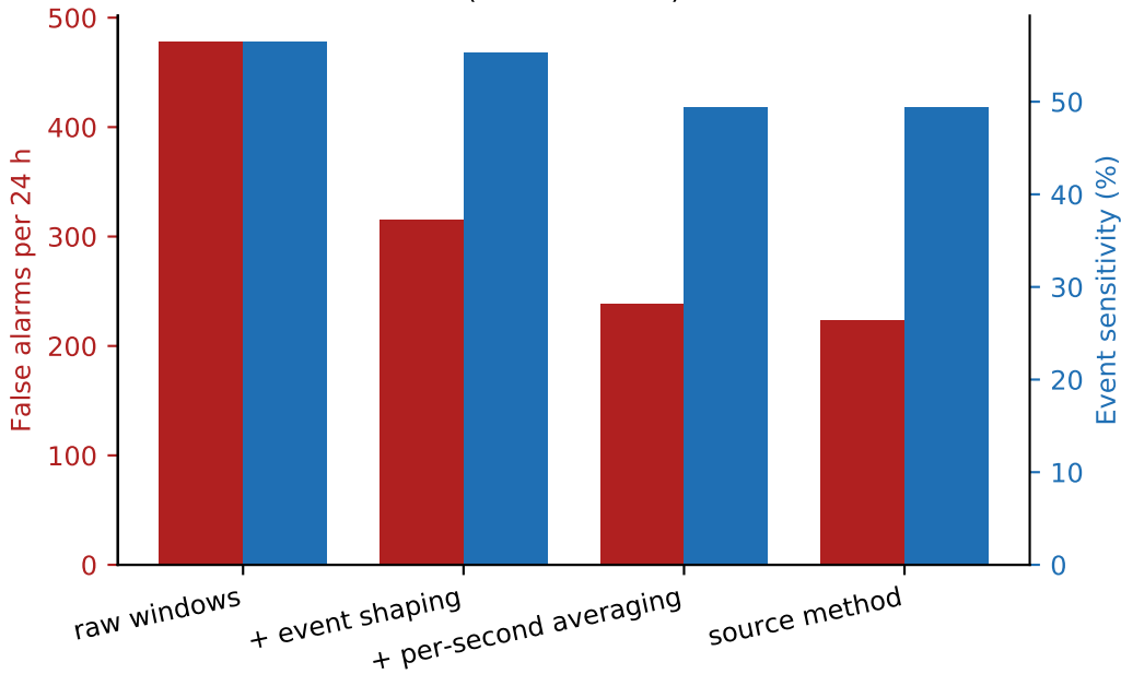
The decision stage, not the model, cuts false alarms 2.1x (threshold 0.5)
