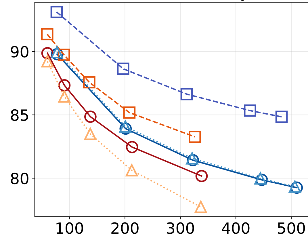
Magnetic Reconnection
