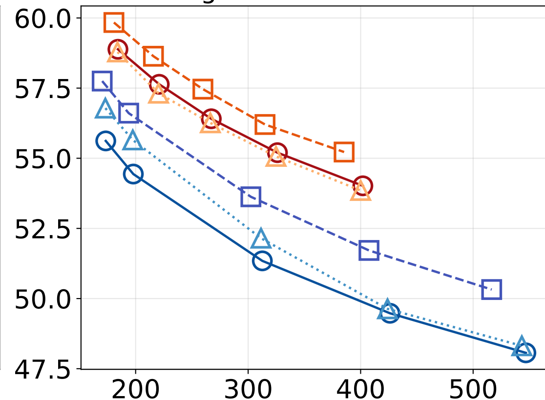
Magnetic Reconnection
