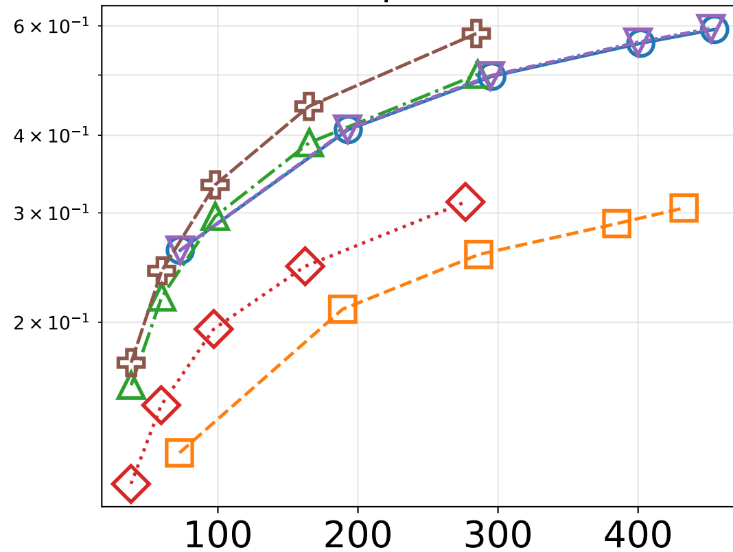
WarpX
