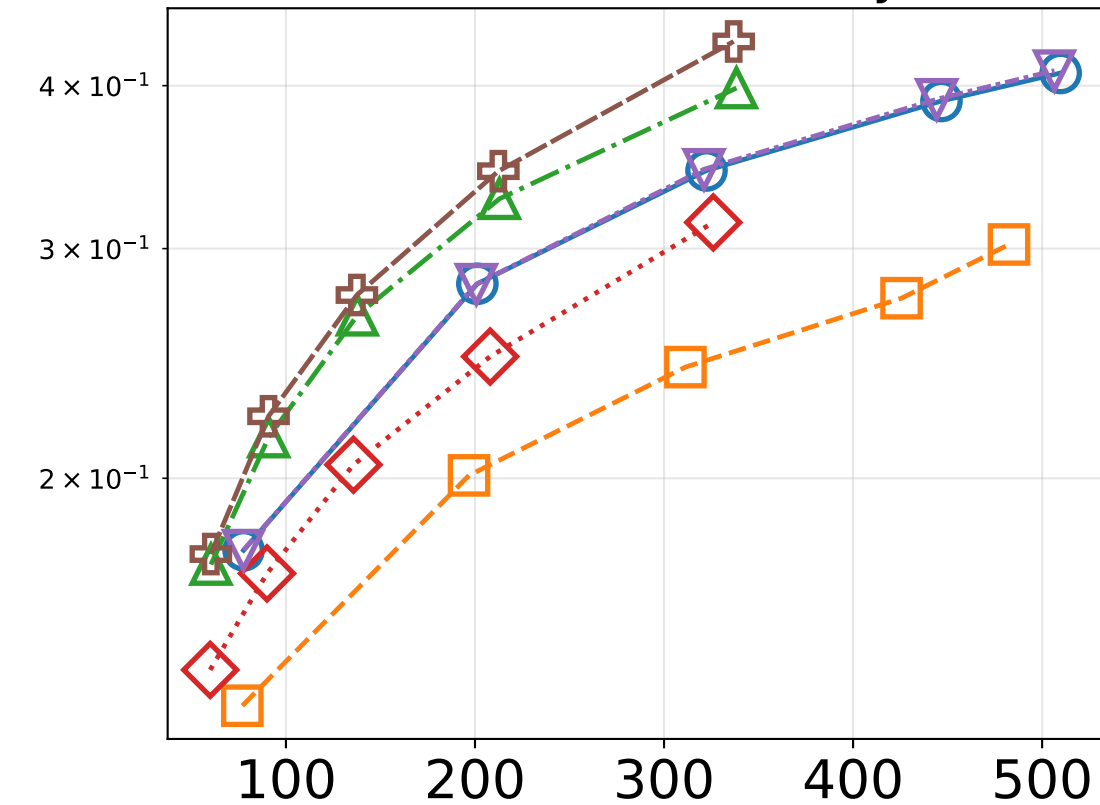
Magnetic Reconnection
