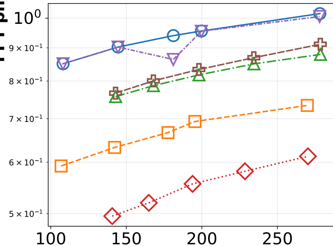
Miranda 1024 3
