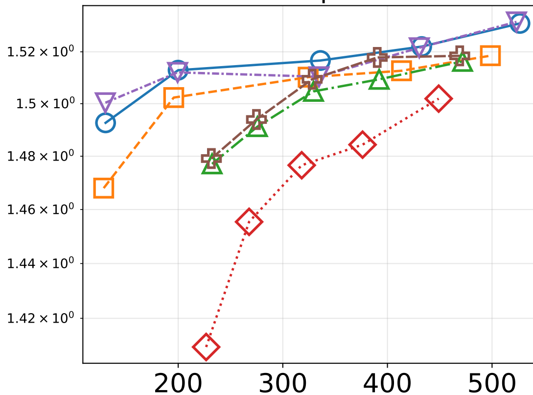
WarpX
