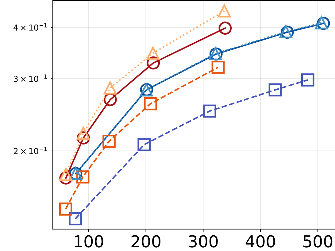
Magnetic Reconnection
