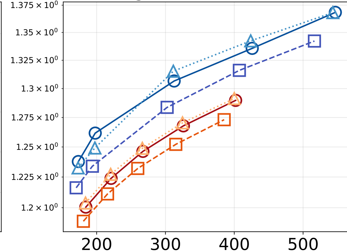
Magnetic Reconnection
