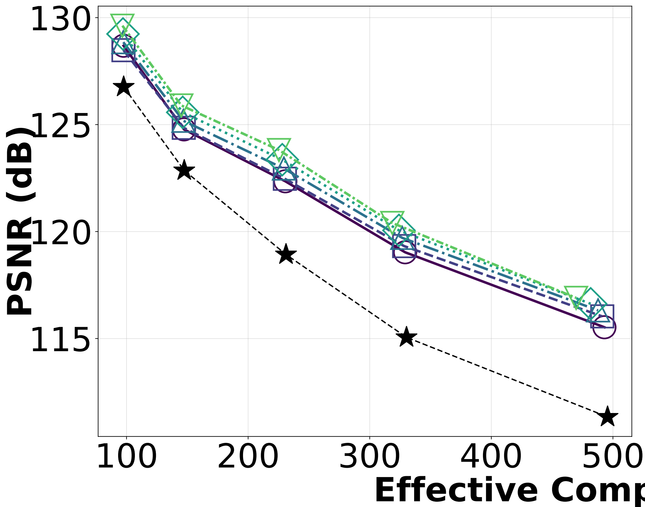
NYX baryon density
