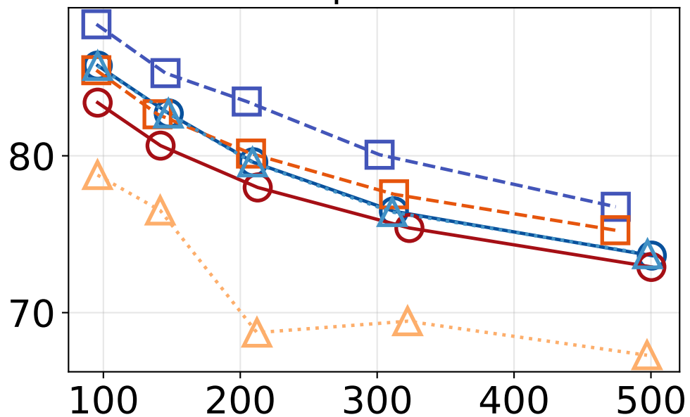
Miranda
