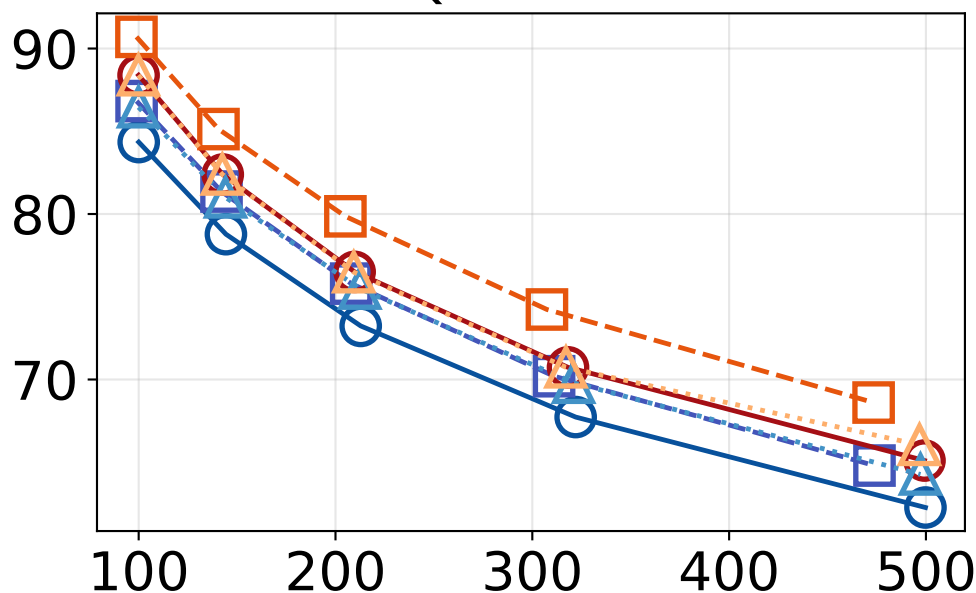
QMCPack
