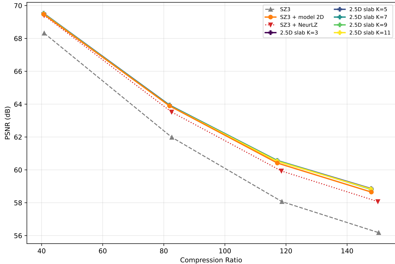
Magnetic Reconnection 512^3 — 2.5D slab depth (iso-time)
