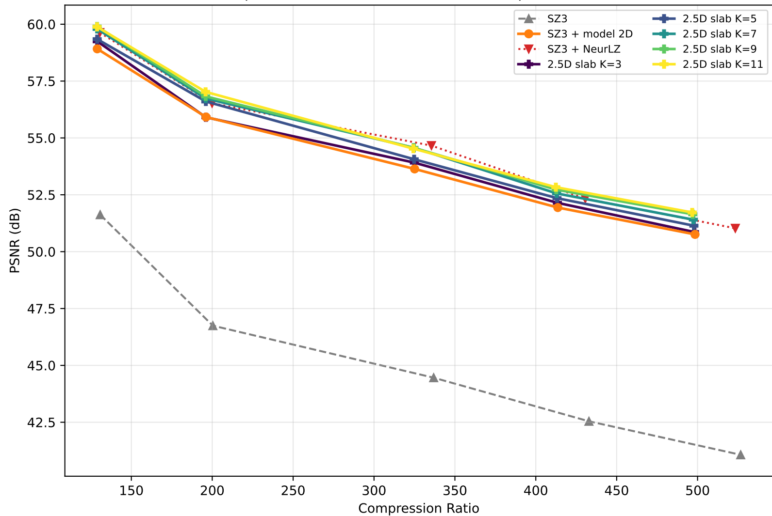
WarpX 2048×256×256 — 2.5D slab depth (iso-time)
