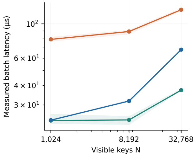
(b) 32 queries, shared K/V
