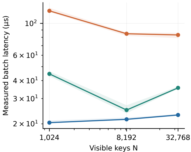
(a) One decode query
