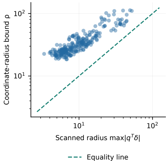
(b) Full-rank score-radius bounds
