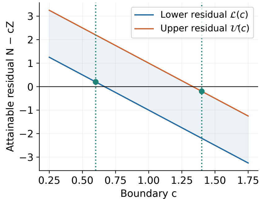
Two signs determine the observation
