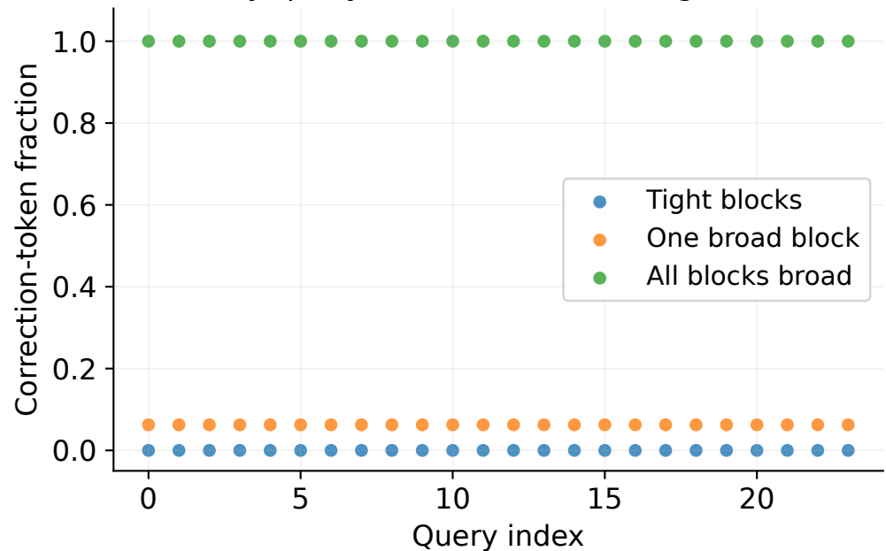
Every query is retained, including failures
