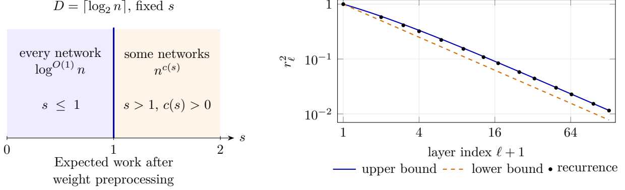
Figure 2: The row-norm threshold and the critical radius. Left: s bounds the absolute row sums. At logarithmic depth, the original preprocessing budget gives polylogarithmic sampling for s \leq 1 ; every fixed s > 1 permits a polynomial lower-bound family. The leading supercritical exponents remain unmatched. Right: both axes are logarithmic, displaying the proved bounds 1/(\ell + 1) \leq r_\ell^2 \leq 3/(2\ell + 3) across the depth range. The black dots are numerical values of r_0 = 1, r_{\ell+1} = \tanh r_\ell ; no proof uses them.
