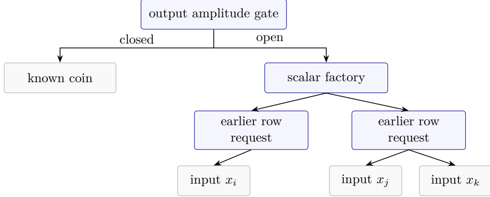
Figure 3: One possible request tree. Only reached calls incur work. A factory may request a random number of earlier signs; the two children shown here are one realization. Each call uses fresh randomness, so predictable charging bounds total work. At fixed input rank, the critical sampler uses the composite function through a precomputed coefficient oracle.
