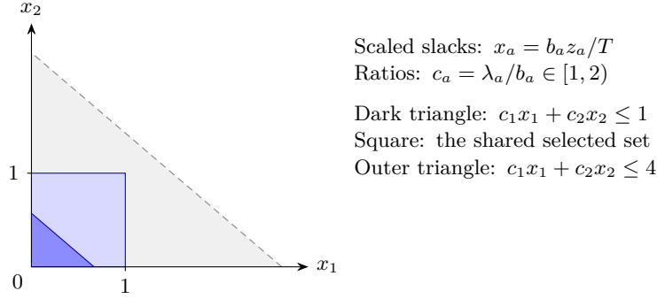
177 Figure 1 The local cap rule in two coordinates, drawn for c_1 = 3/2 and c_2 = 7/4 . Nonnegative 178 coordinates put the true T -cap inside the unit square. The square is fixed throughout the bin and 179 has deficit below 4T . With three coordinates the same argument gives 6T .
