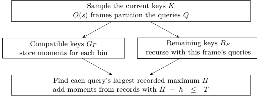
254 Figure 2 At each node a query uses one frame. Its compatible keys contribute a summary; its 255 remaining keys follow one recursive path. The recorded pieces are disjoint even though other queries 256 may use different pieces.
