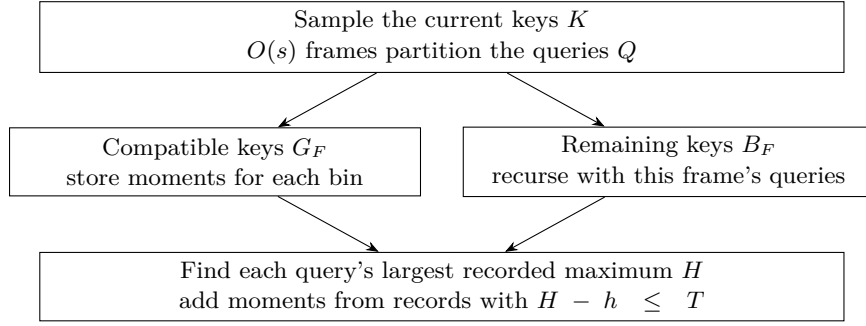
241 ■ Figure 2 At each node a query uses one frame. Its compatible keys contribute a summary; its 242 remaining keys follow one recursive path. The recorded pieces are disjoint even though other queries 243 may use different pieces.
