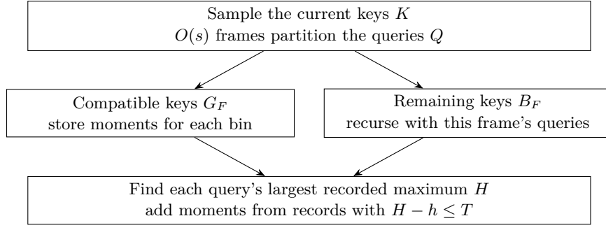
255 Figure 2 At each node a query uses one frame. Its compatible keys contribute a summary; its 256 remaining keys follow one recursive path. For each query the recorded pieces are disjoint. Other 257 queries may use different pieces.
