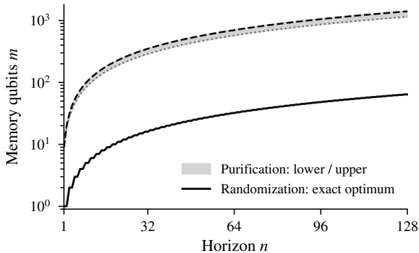
(a) Return tolerance \delta = 0.1
