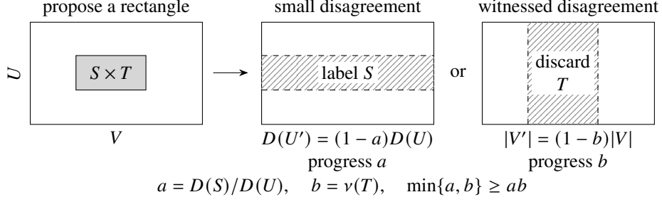
Figure 1: An accepted proposal either removes a fraction a of the remaining point mass or a fraction b of the surviving hypotheses. The shaded band marks what is removed. Both updates have progress at least ab , the quantity controlled by the pointwise rectangle mixture.
