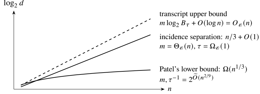
Figure 3: Growth orders of log dimension at fixed learning and representation errors; constants are suppressed. The incidence bound holds for all three dimension notions and meets the exponential order of the transcript bound at its own query resources. The dashed line uses K = Q = 2^n , m = \Theta_\varepsilon(n) , and fixed tolerance; it is not the upper bound at Patel’s resources. Patel’s curve denotes an ordinary-dimension lower bound, not an upper bound on his class.
